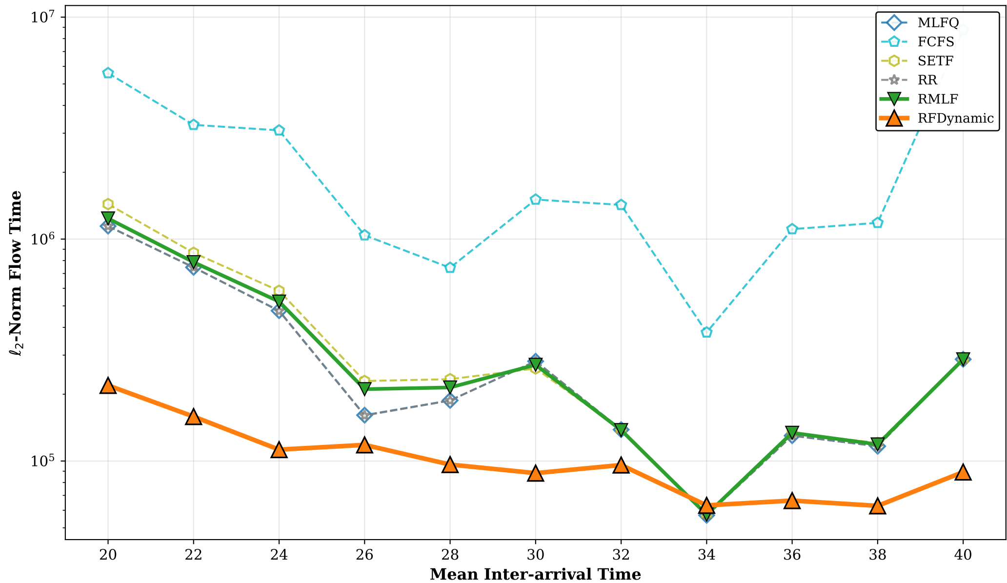
Non-Clairvoyant \ell_2 -Norm Comparison Bounded Pareto ( H = 2^{18} , H/L \approx 64359 )
