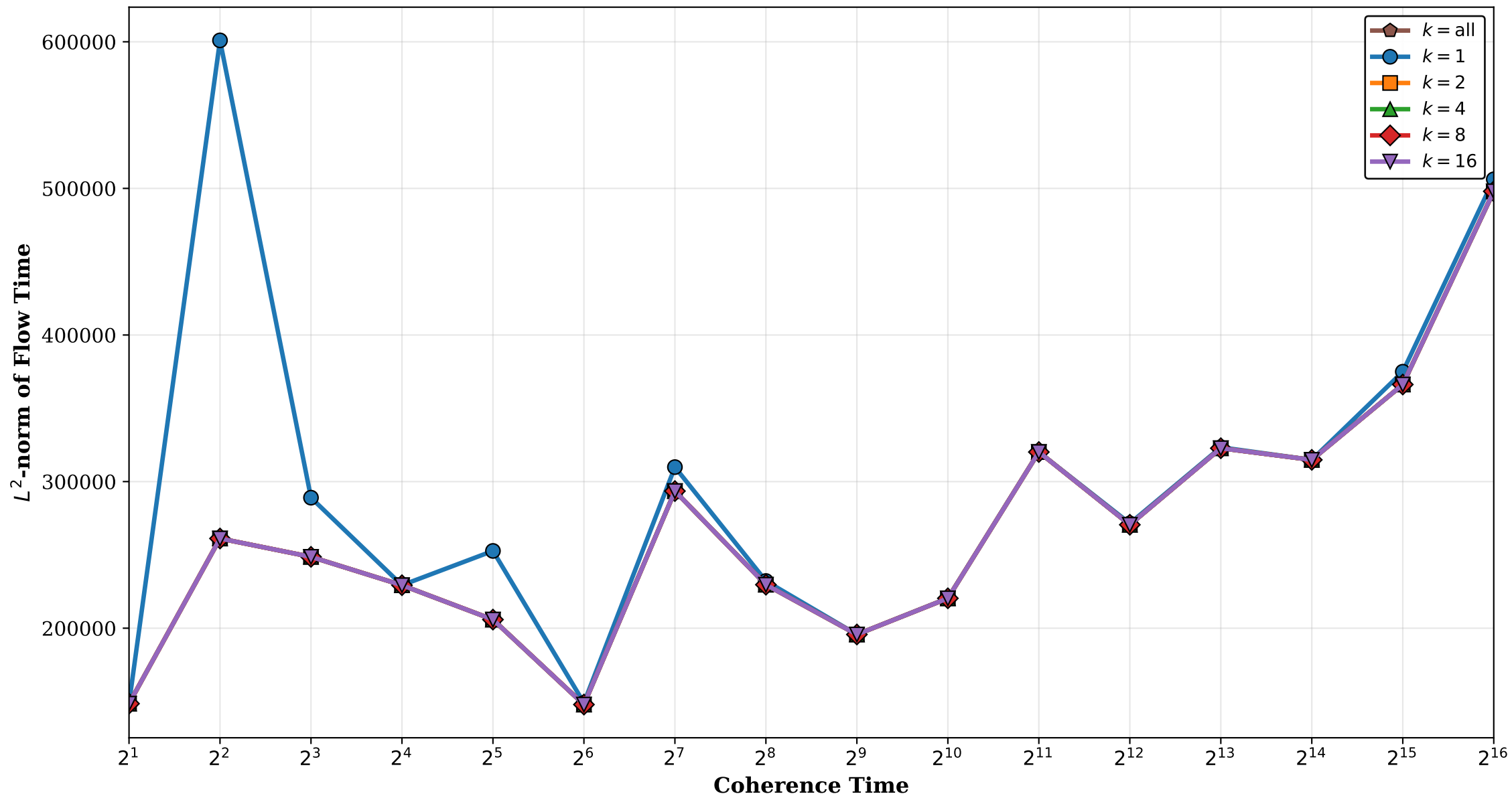
Dynamic Lookback Comparison Soft Random ( H = 2^{12}, 2^{15}, 2^{18} )
