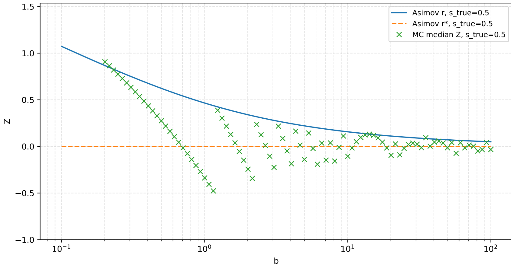
Asimov vs MC median Z, s_{\text{true}} = 0.5
