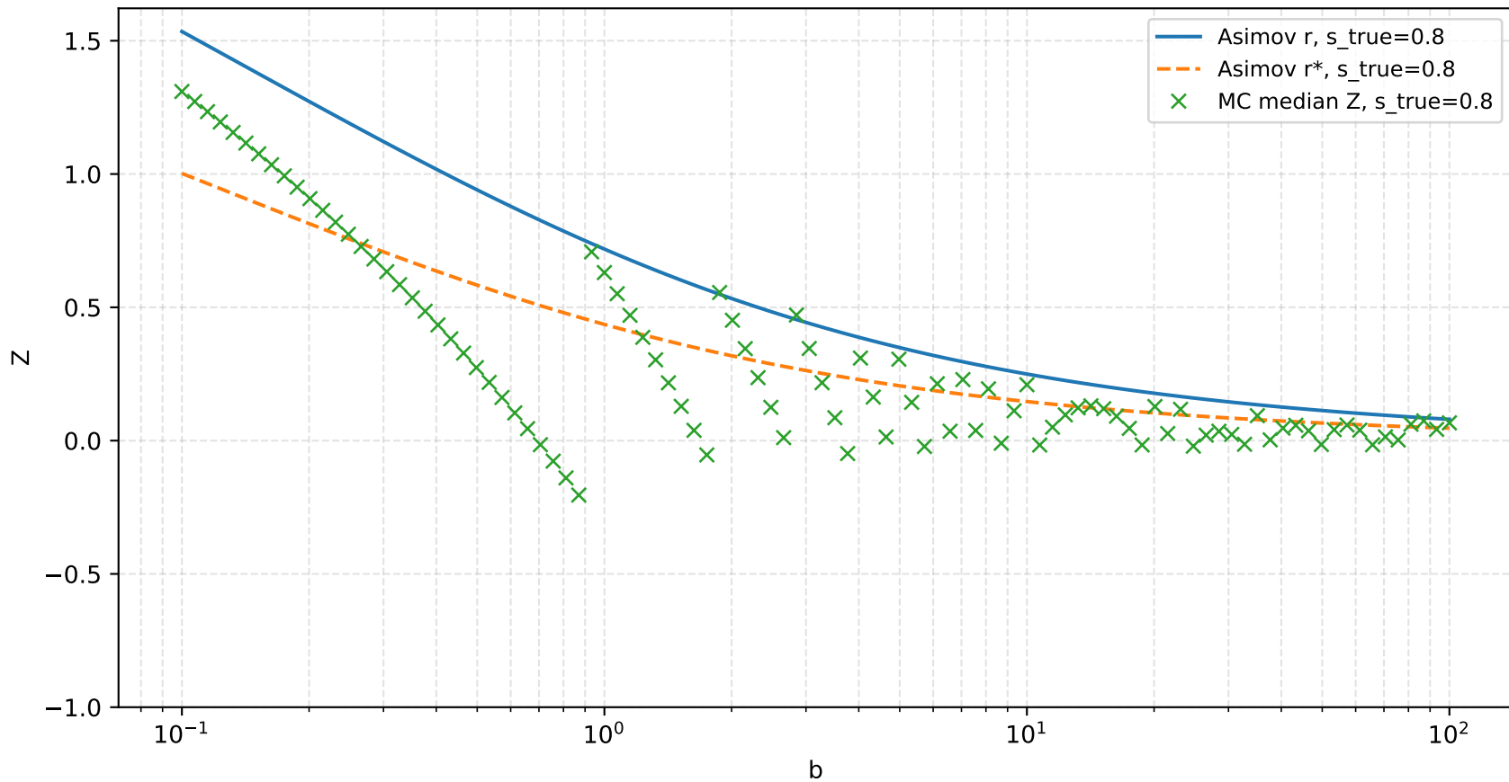
Asimov vs MC median Z, s_{\text{true}} = 0.8
