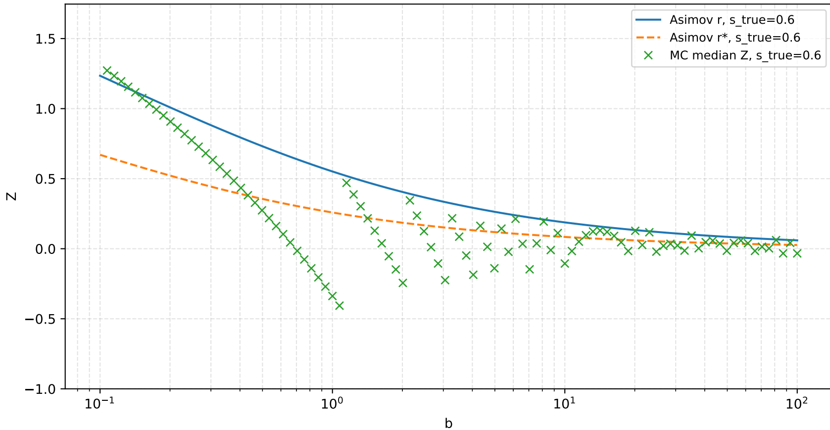
Asimov vs MC median Z, s_{\text{true}} = 0.6
