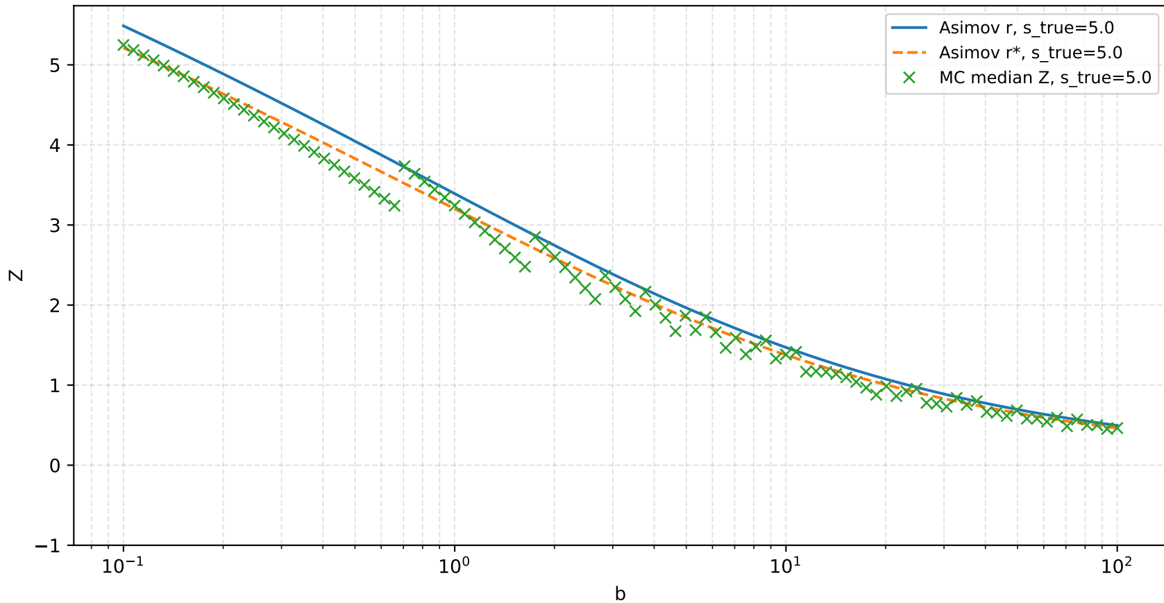
Asimov vs MC median Z, s_{\text{true}} = 5.0
