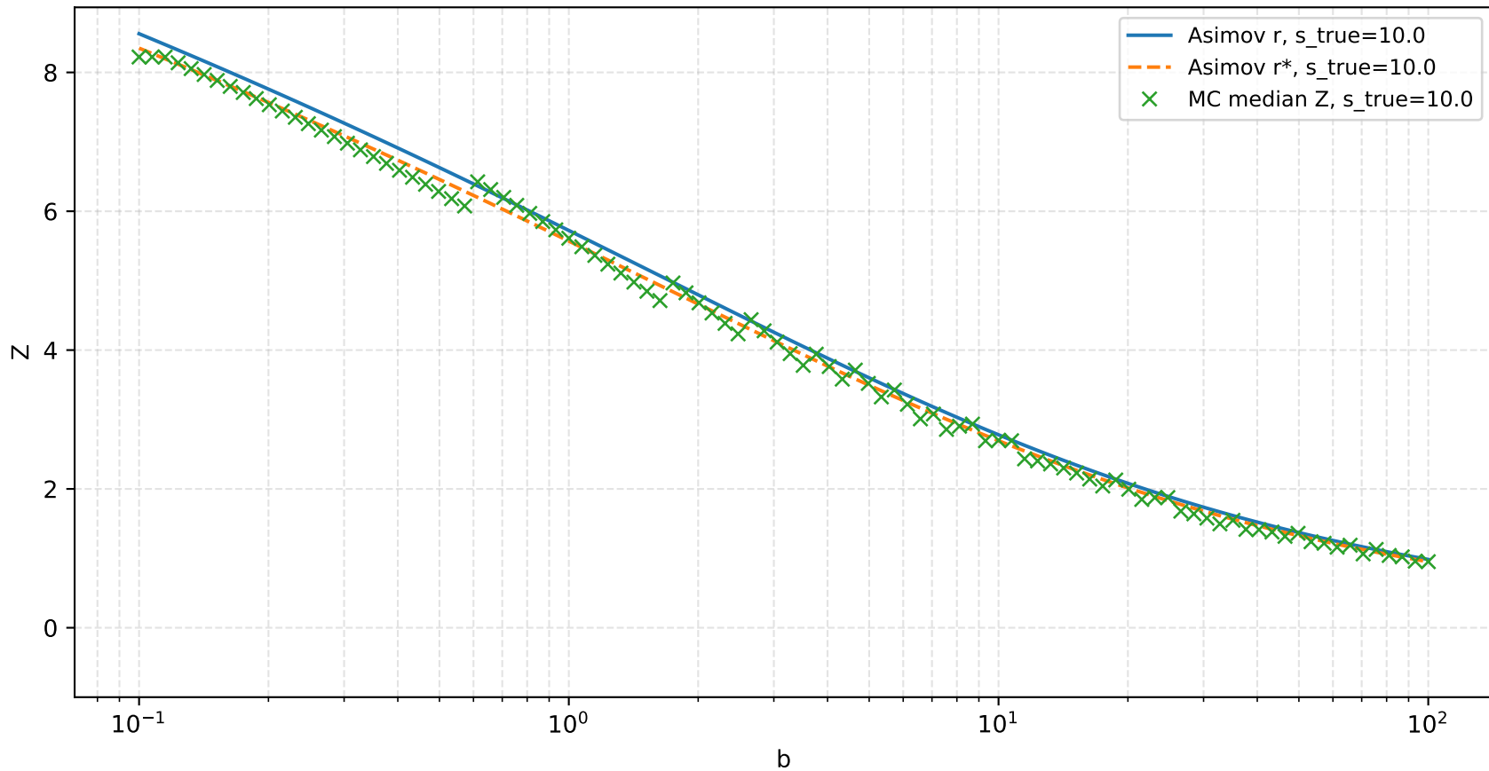
Asimov vs MC median Z, s_{\text{true}} = 10.0
