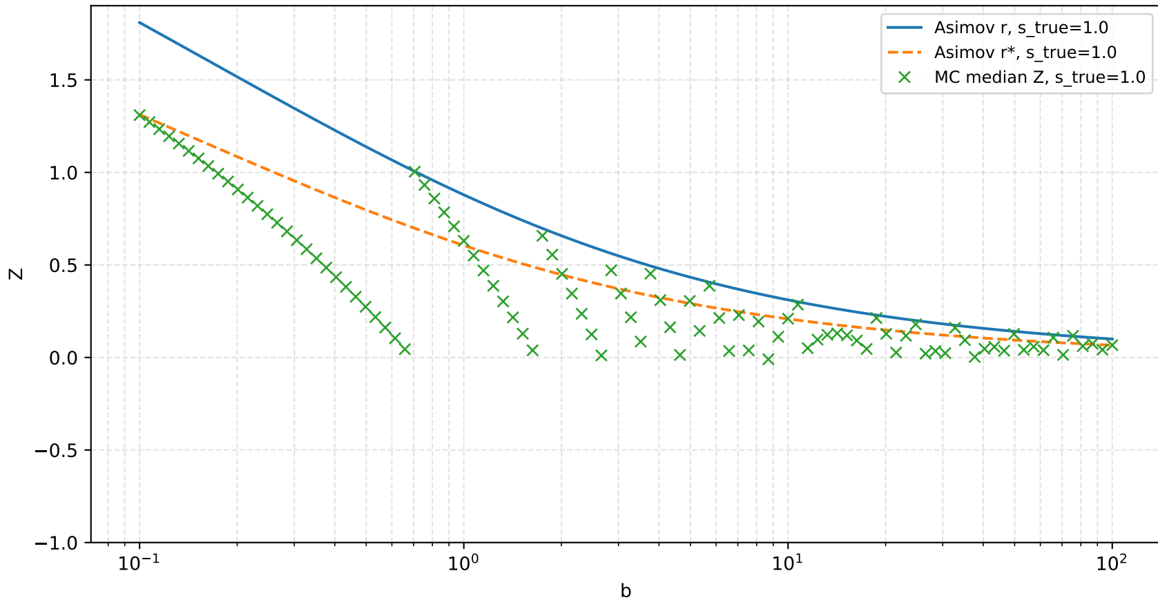
Asimov vs MC median Z, s_{\text{true}} = 1.0
