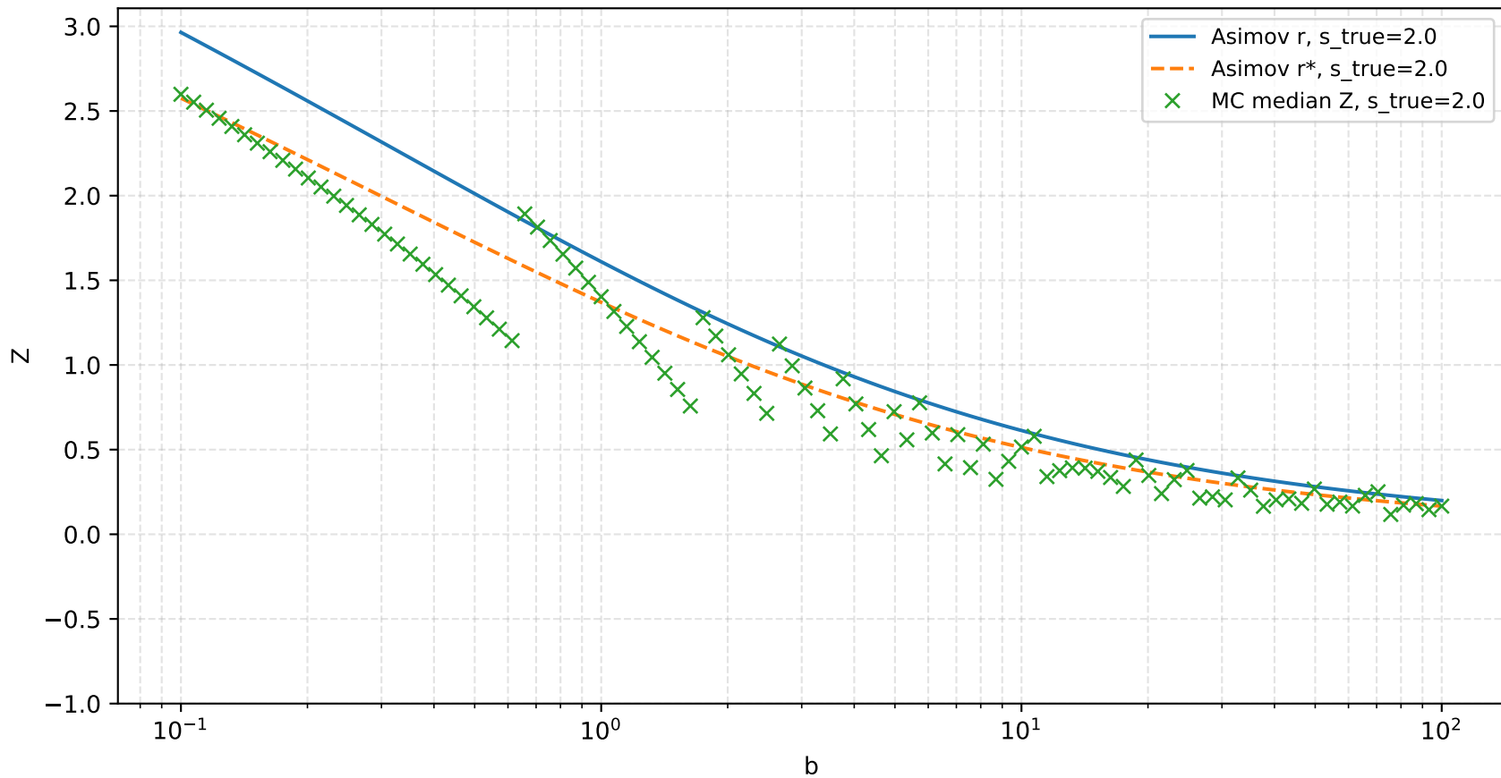
Asimov vs MC median Z, s_{\text{true}} = 2.0
