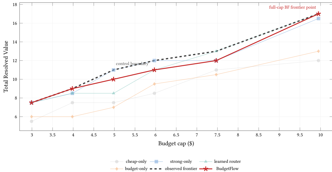
Figure 2: Budget sensitivity diagnostic on the 5-policy Value-Aware Budget Flow case. Outcomes are fixed; budget accounting is replayed at alternate caps without re-planning task order or routing. The dashed line is the observed frontier; BudgetFlow is emphasized in red, while controls are shown as lighter diagnostic curves.
