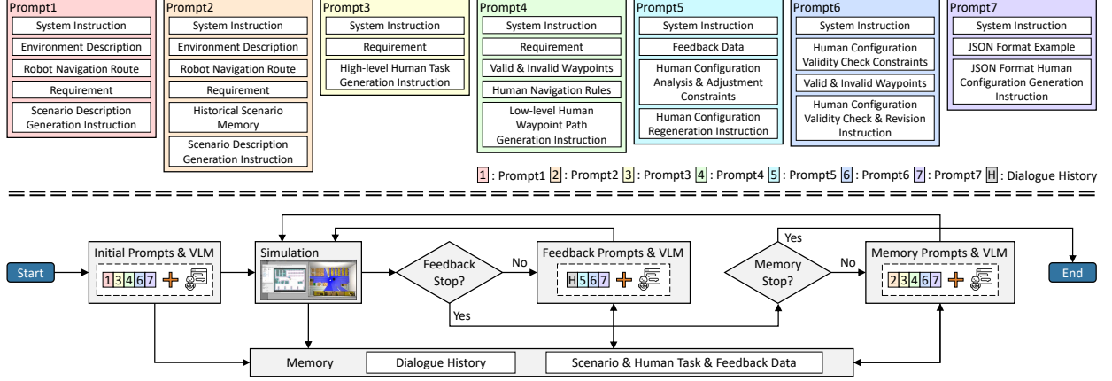
Figure 3: Prompt templates for multi-turn conversations and scenario generation workflow with feedback and memory in RVSG.
