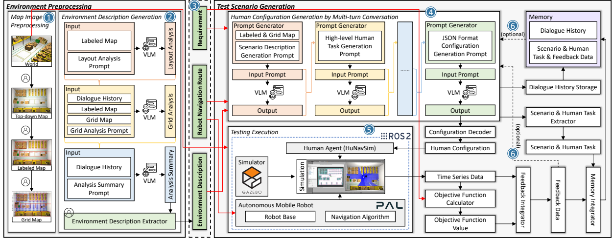
Figure 2: Overview of RVSG during the iterative testing of autonomous mobile robots.
