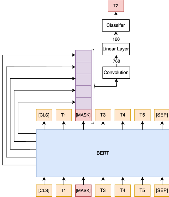
Figure 1. Updated version of text model
