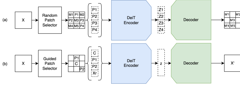
Figure 2. (a) Second iteration of the image model P\# denotes the selected patches, M\# denotes the masked patches (b) Final iteration of the image model P\# denotes the selected patches, C is the center patch, Xr is resized image
