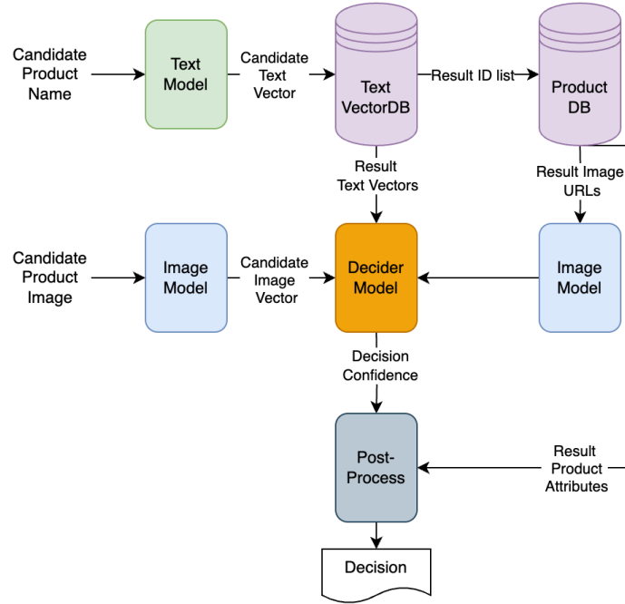
Figure 3. Final system design for product deduplication.
