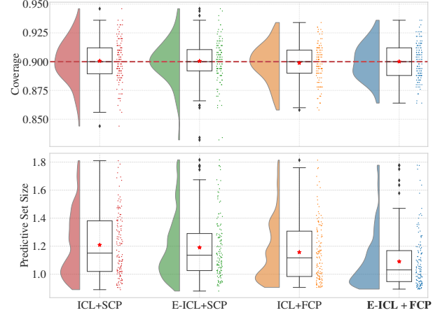
Fig. 3. Coverage probability and predictive set size achieved by ICL-based schemes on the image classification tasks (★ marks the mean, \alpha = 0.1 ).
