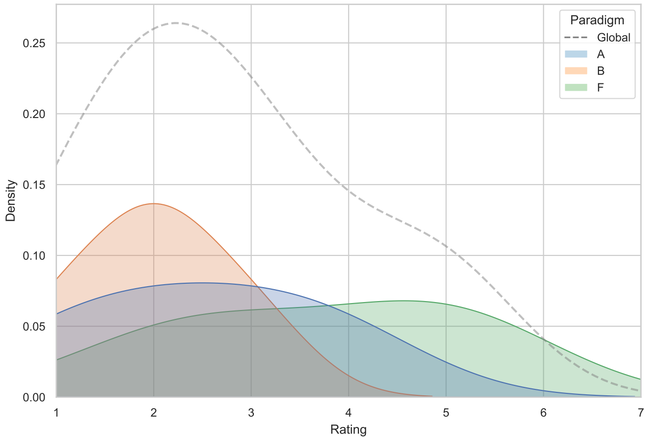
Culture_Closeness_Q3 | Global_Paradigm
