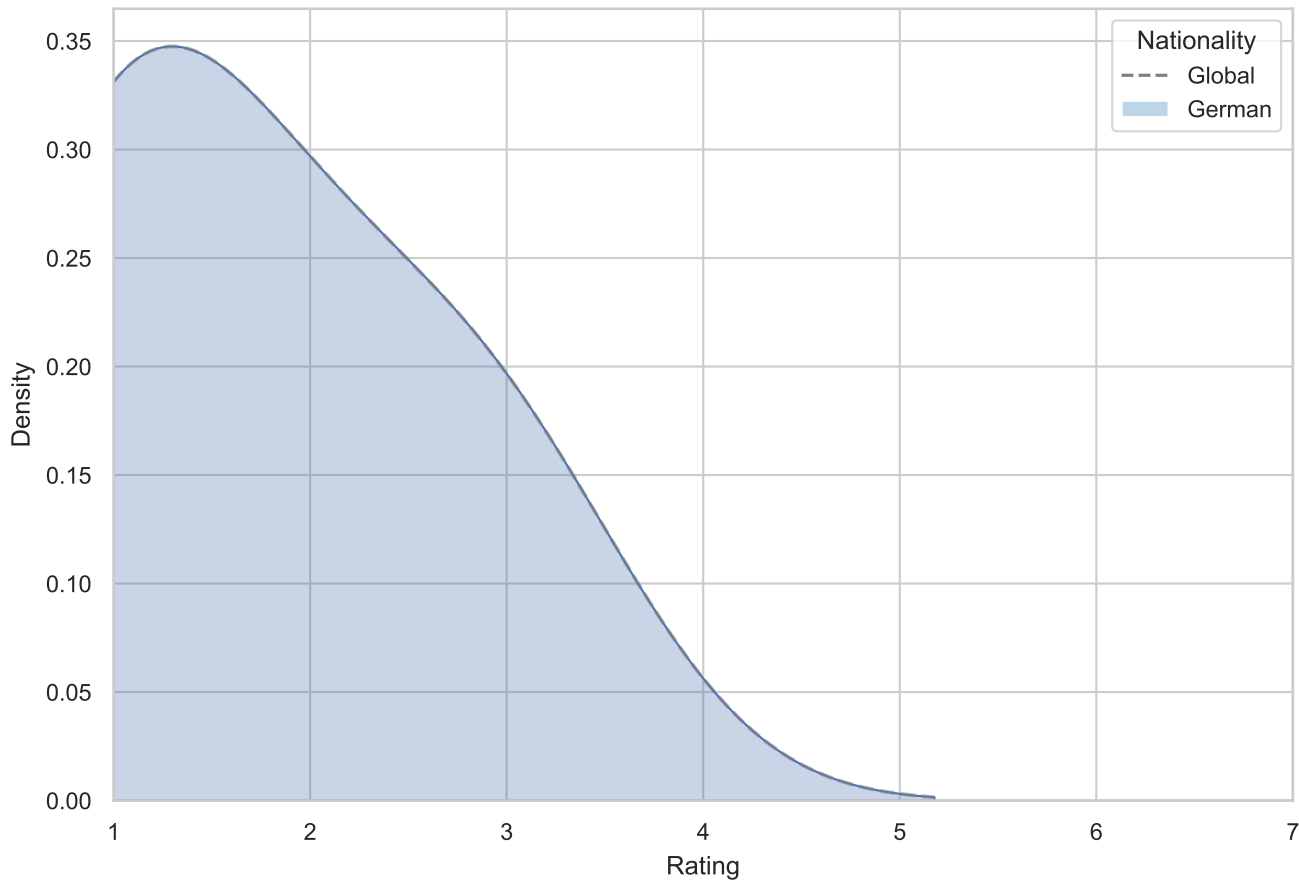
Culture_Closeness_Q1 | Paradigm_A_Nationality
