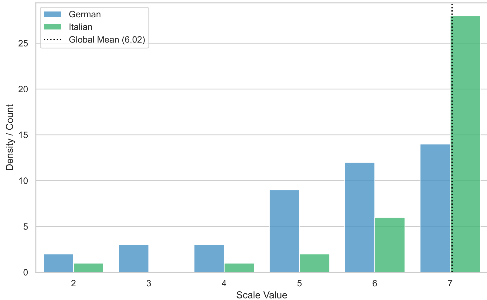
Distribution Comparison: Culture Affinity Q2
