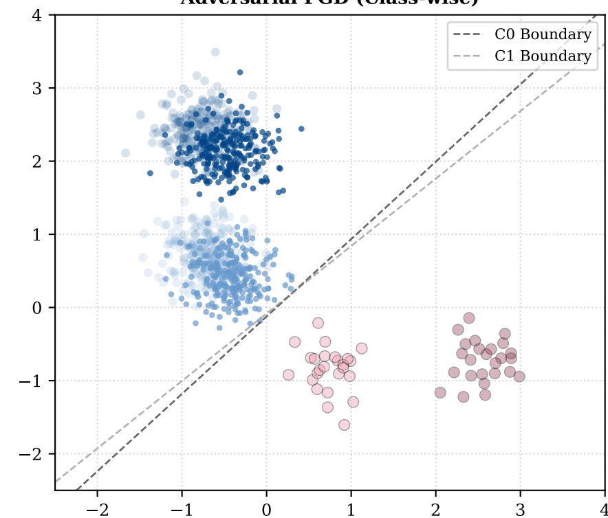
Adversarial PGD (Class-wise)
