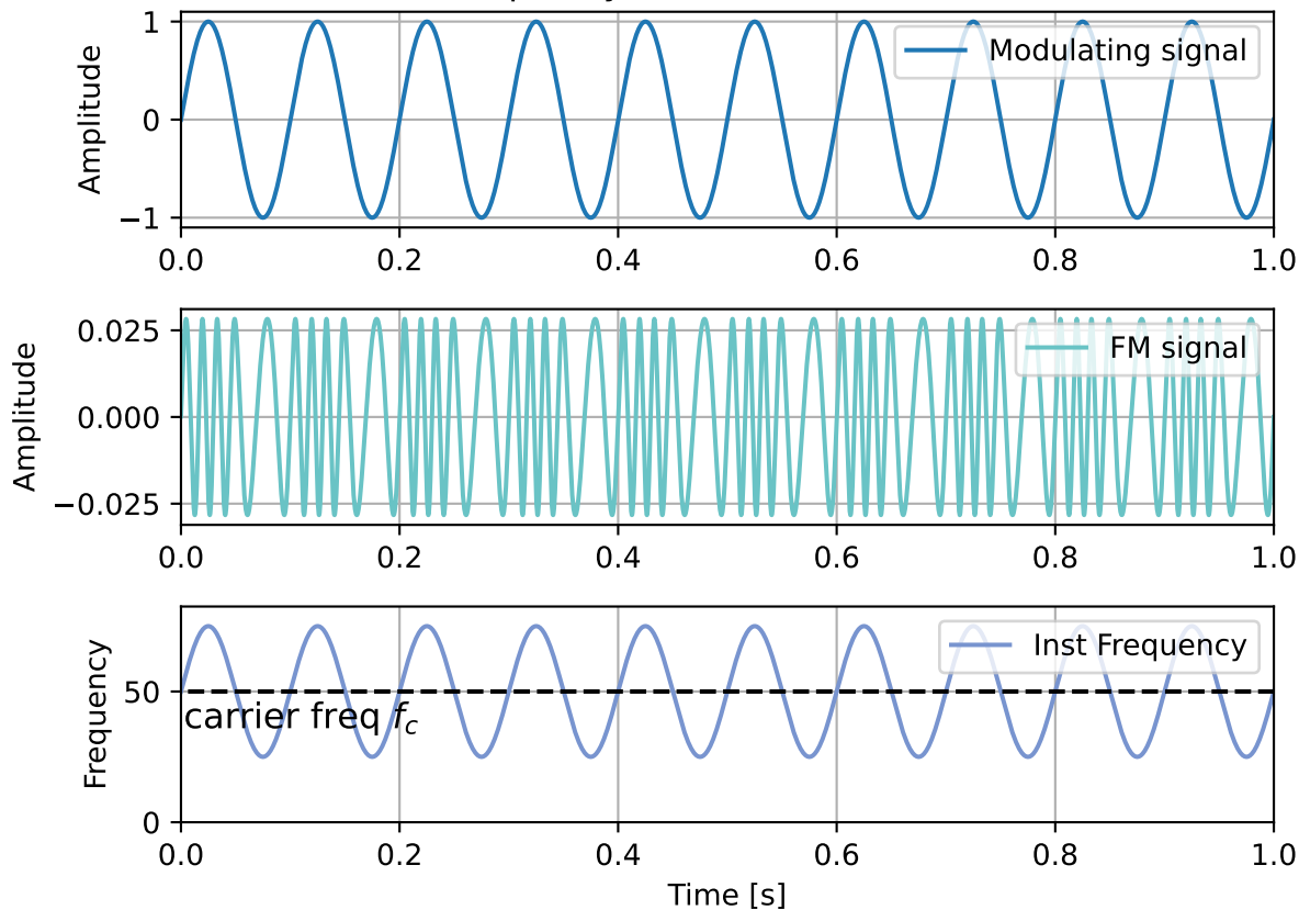
Frequency-modulated sine wave
