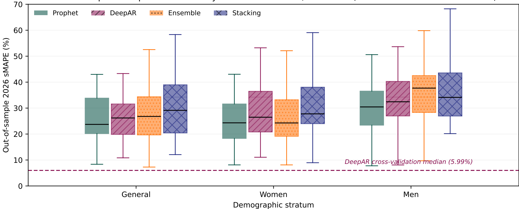
Out-of-sample 2026 per-series error by model and stratum, W02-W18 (each box: 32 entities + national)
