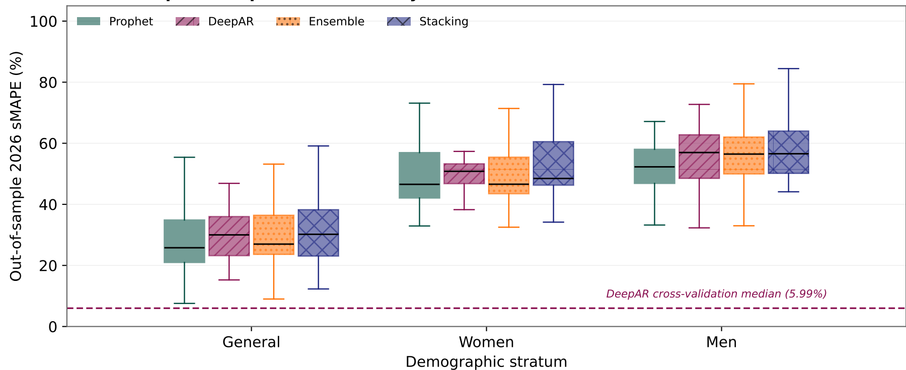
Out-of-sample 2026 per-series error by model and stratum (each box: 32 entities + national)
