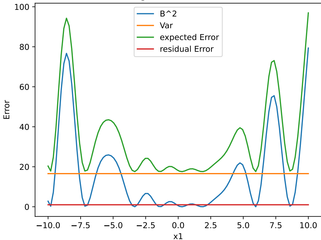
kNN Regression Bias-Variance
