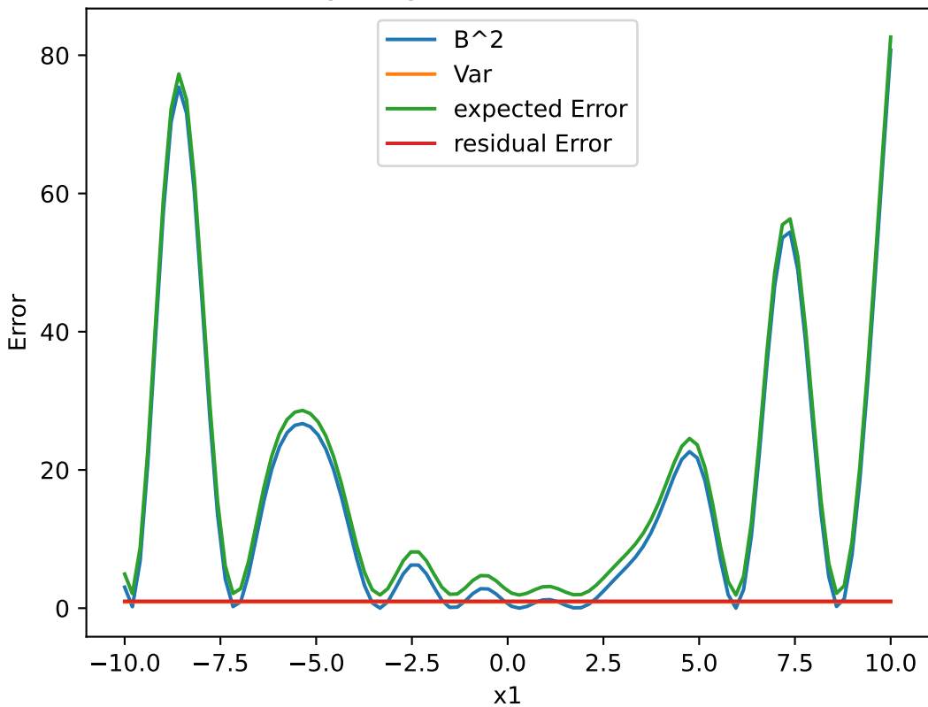
ridge Regression Bias-Variance
