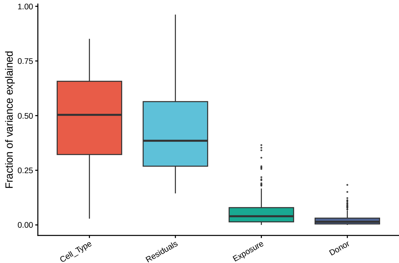
TF-activity variance: lineage vs exposure vs donor
