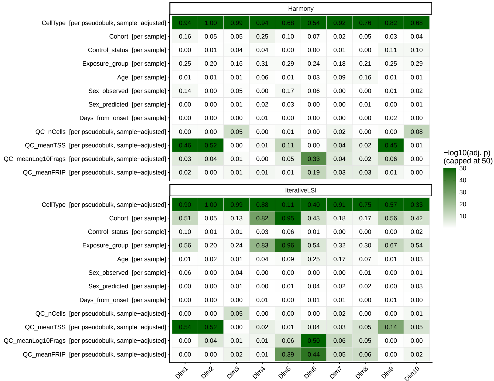
Association of pseudobulk (sample x cell type) dimensions with covariates
