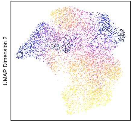
UMAP_HIV of IterativeLSI_hiv colored by GeneScoreMatrix : IL2RA
