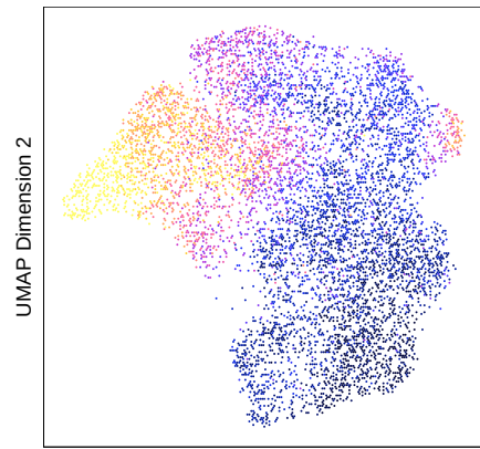
UMAP_HIV of IterativeLSI_hiv colored by GeneScoreMatrix : TIGIT
