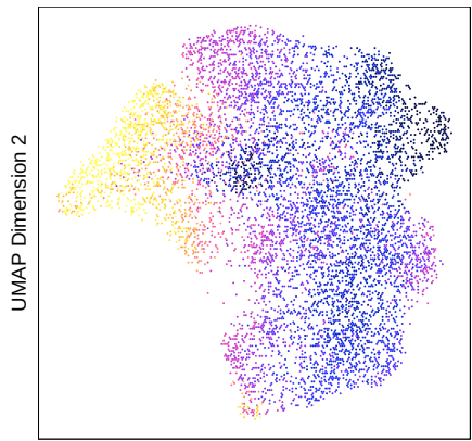
UMAP_HIV of IterativeLSI_hiv colored by GeneScoreMatrix : ROBO1
