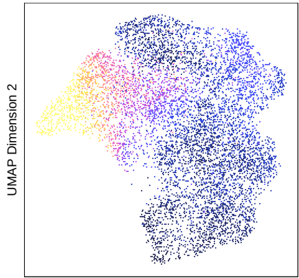
UMAP_HIV of IterativeLSI_hiv colored by GeneScoreMatrix : CD8B
