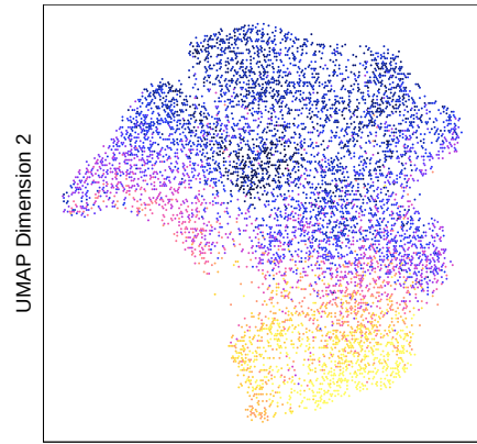
UMAP_HIV of IterativeLSI_hiv colored by GeneScoreMatrix : CD4
