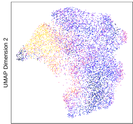
UMAP_HIV of IterativeLSI_hiv colored by GeneScoreMatrix : ROBO2
