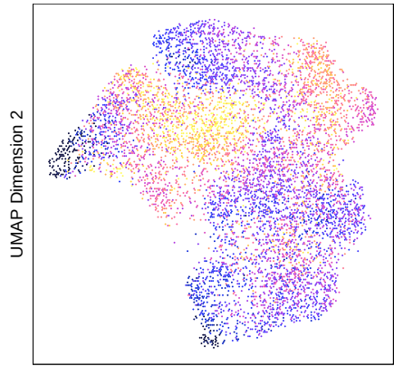
UMAP_HIV of IterativeLSI_hiv colored by GeneScoreMatrix : FOXP3
