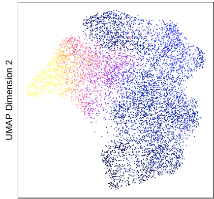
UMAP_HIV of IterativeLSI_hiv colored by GeneScoreMatrix : CD8A
