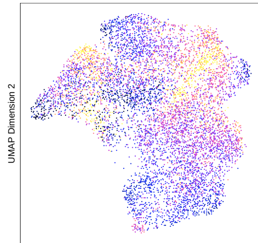
UMAP_HIV of IterativeLSI_hiv colored by GeneScoreMatrix : CD4
