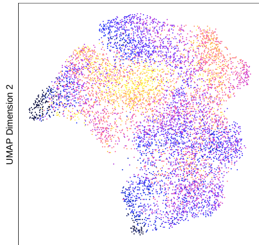
UMAP_HIV of IterativeLSI_hiv colored by GeneScoreMatrix : FOXP3
