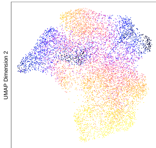
UMAP_HIV of IterativeLSI_hiv colored by GeneScoreMatrix : IL2RA
