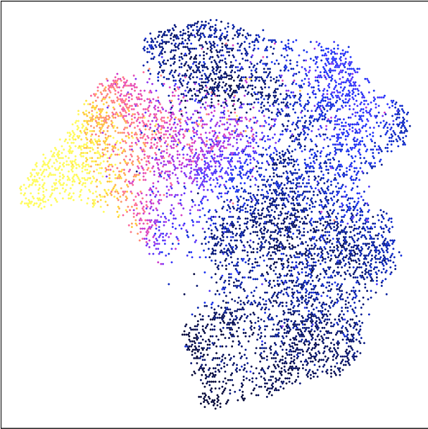
UMAP_HIV of IterativeLSI_hiv colored by GeneScoreMatrix : ROBO1
