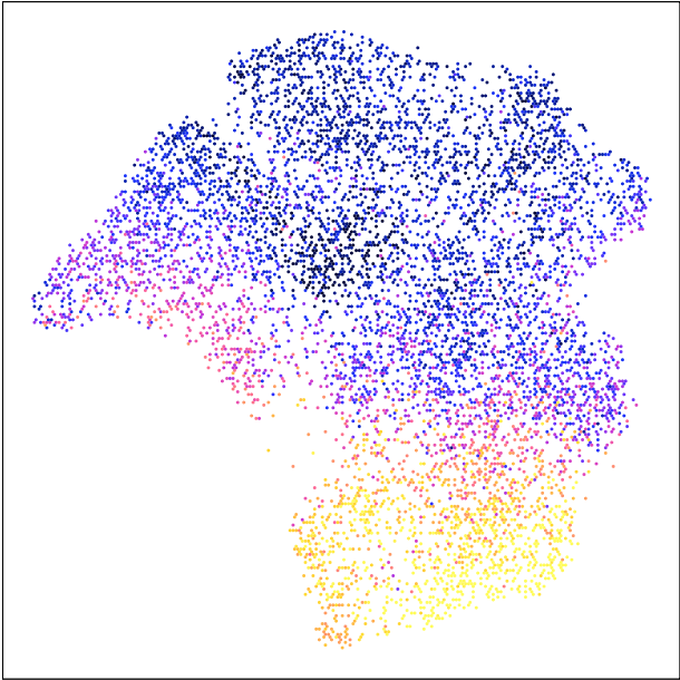
UMAP_HIV of IterativeLSI_hiv colored by GeneScoreMatrix : TIGIT
