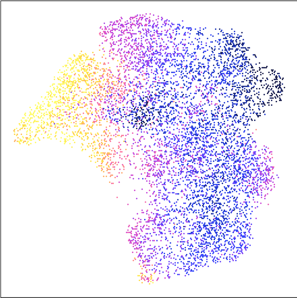
UMAP_HIV of IterativeLSI_hiv colored by GeneScoreMatrix : CTLA4
