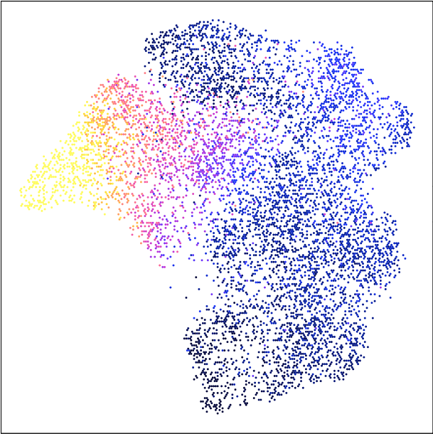
UMAP_HIV of IterativeLSI_hiv colored by GeneScoreMatrix : ROBO2
