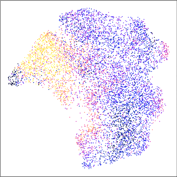
UMAP_HIV of IterativeLSI_hiv colored by GeneScoreMatrix : HAVCR2
