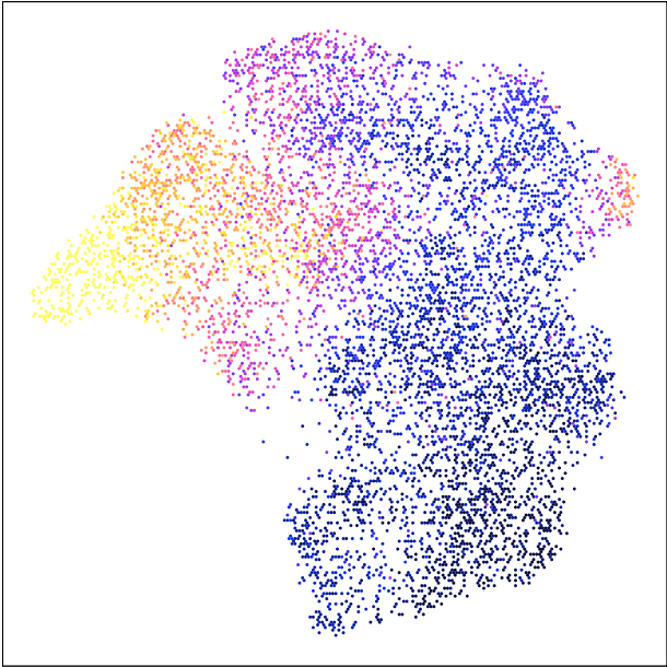
UMAP_HIV of IterativeLSI_hiv colored by GeneScoreMatrix : NCAM1
