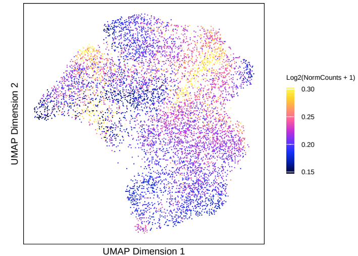
UMAP_HIV of IterativeLSI_hiv colored by GeneScoreMatrix : CD4
