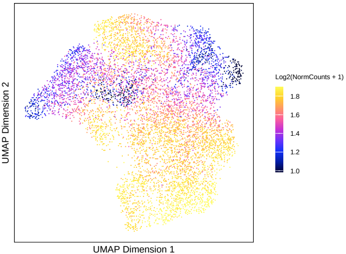
UMAP_HIV of IterativeLSI_hiv colored by GeneScoreMatrix : FOXP3
