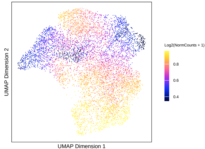
UMAP_HIV of IterativeLSI_hiv colored by GeneScoreMatrix : IL2RA
