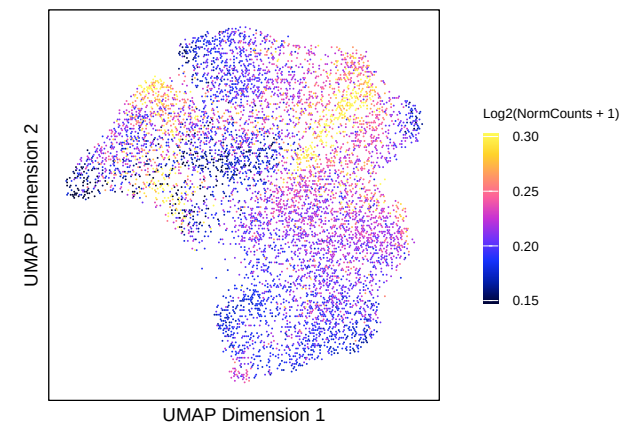
UMAP_HIV of IterativeLSI_hiv colored by GeneScoreMatrix : CD4
