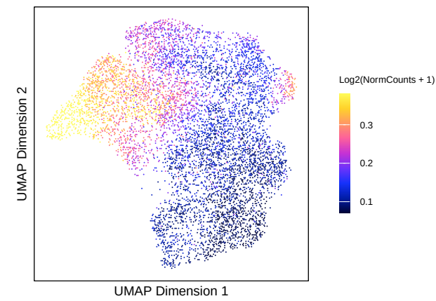
UMAP_HIV of IterativeLSI_hiv colored by GeneScoreMatrix : TIGIT
