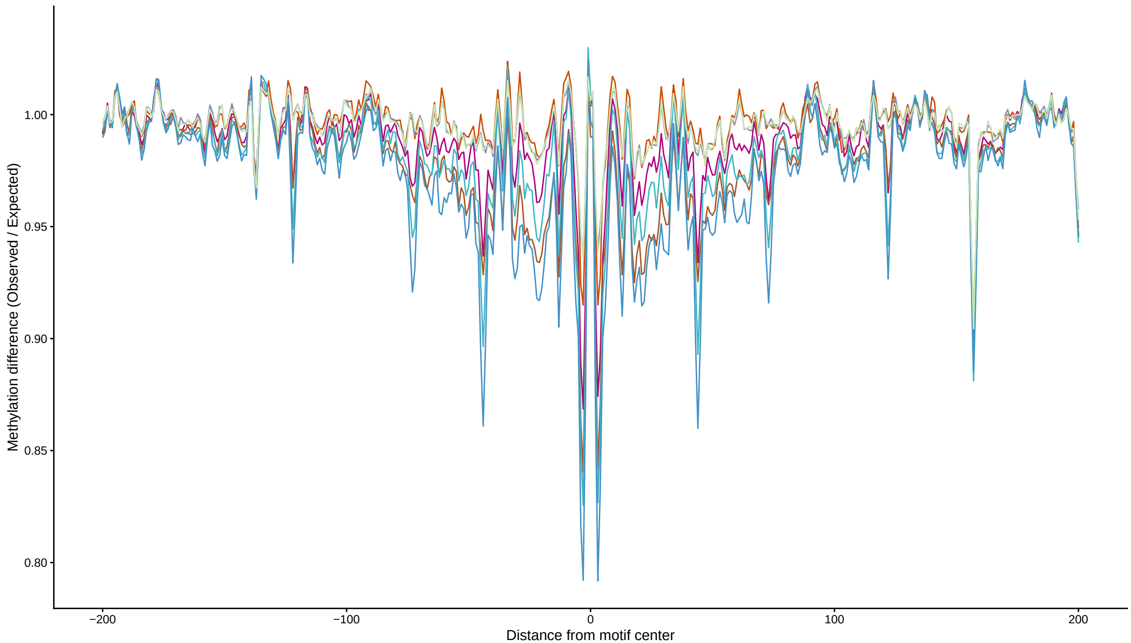
TF footprint difference for TBR1
