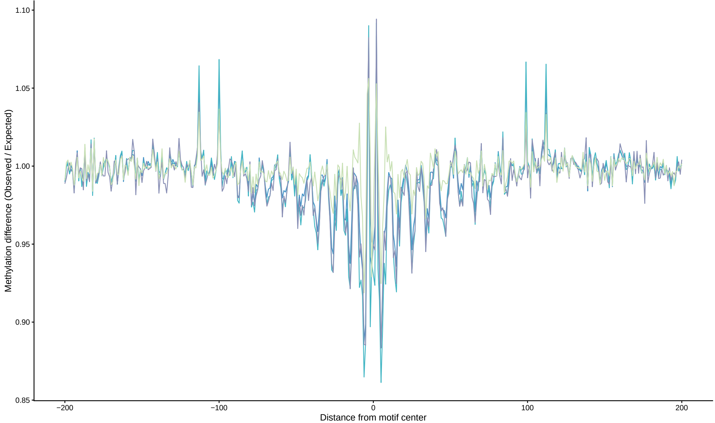
TF footprint difference for EBF1
