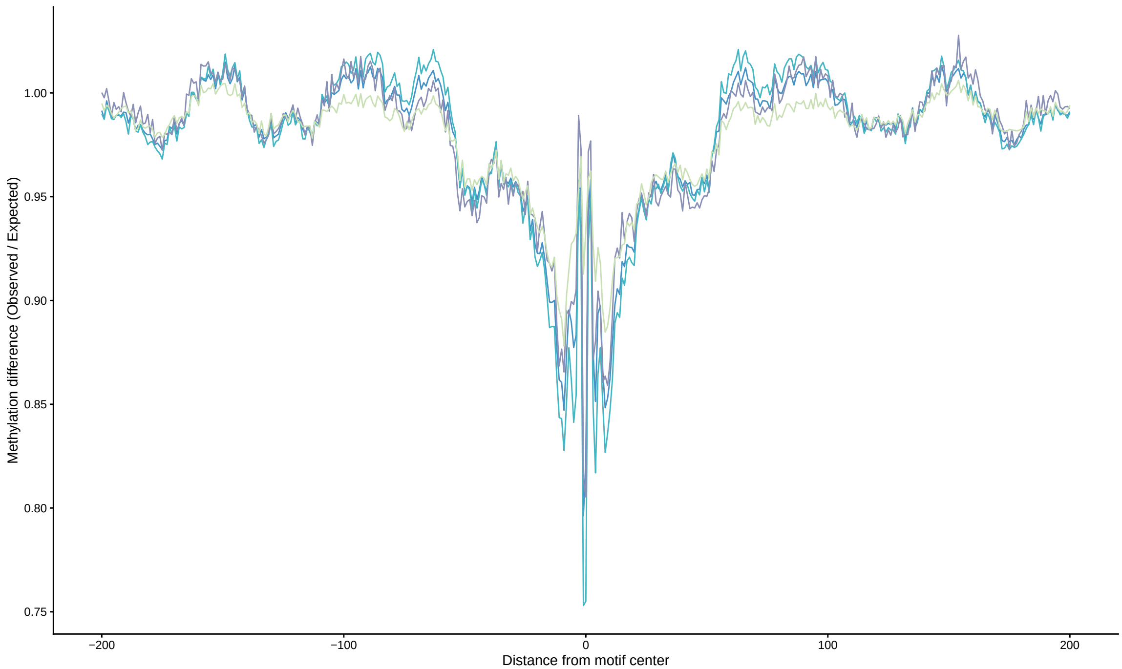
TF footprint difference for SPI1
