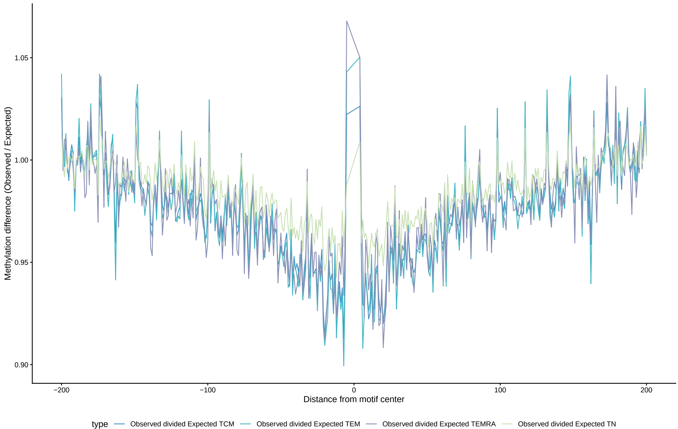
TF footprint difference for TCF7
