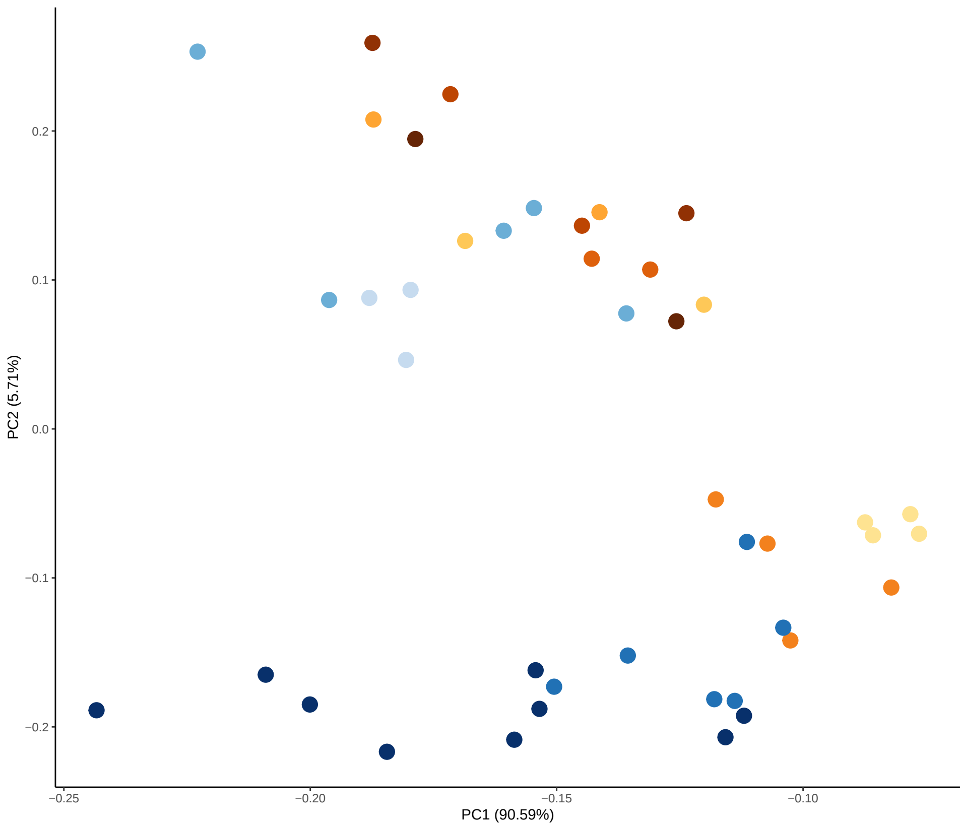
PCA – B-Cell and T-Cell Subsets (No Thymocytes)
