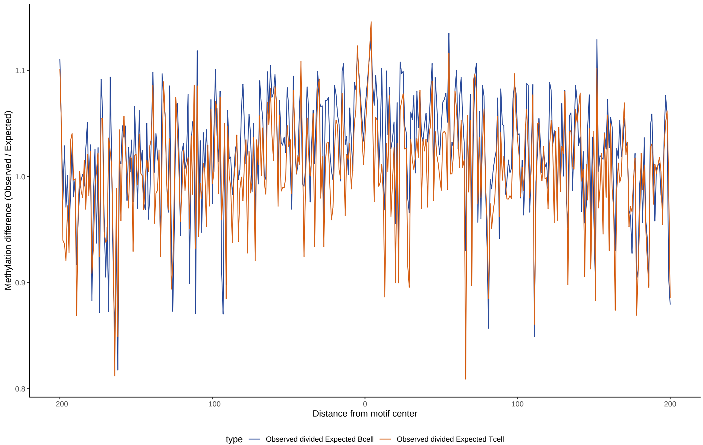
TF footprint difference for CUX2
