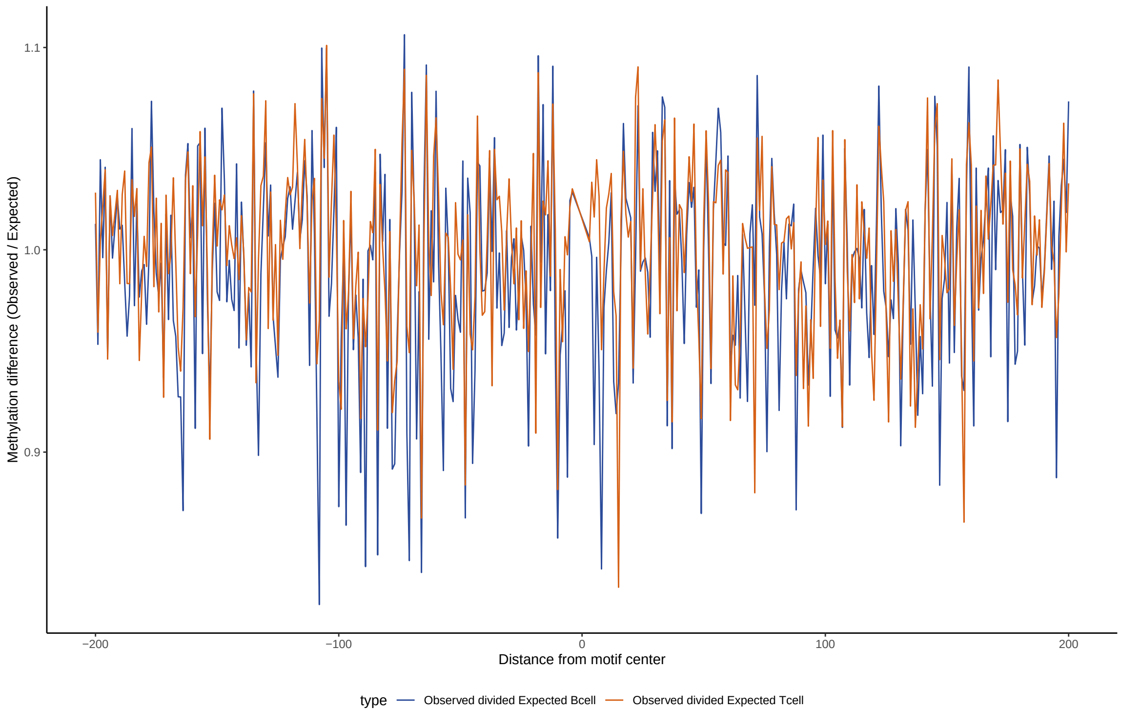
TF footprint difference for LHX1
