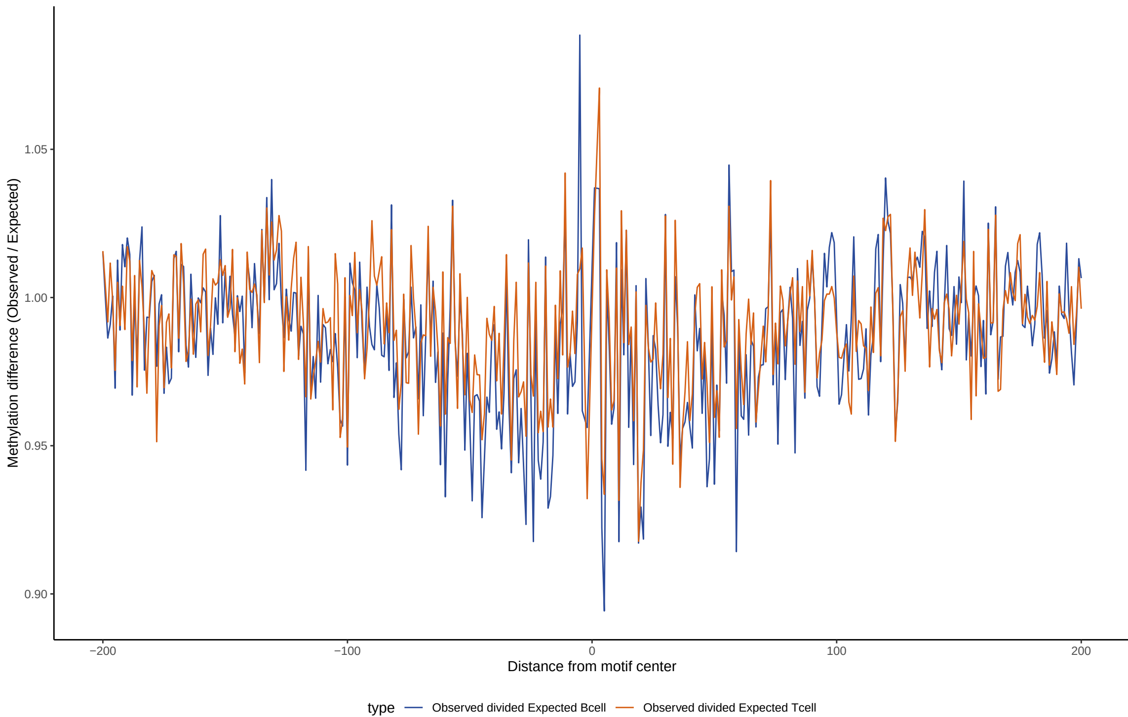
TF footprint difference for ZBTB18
