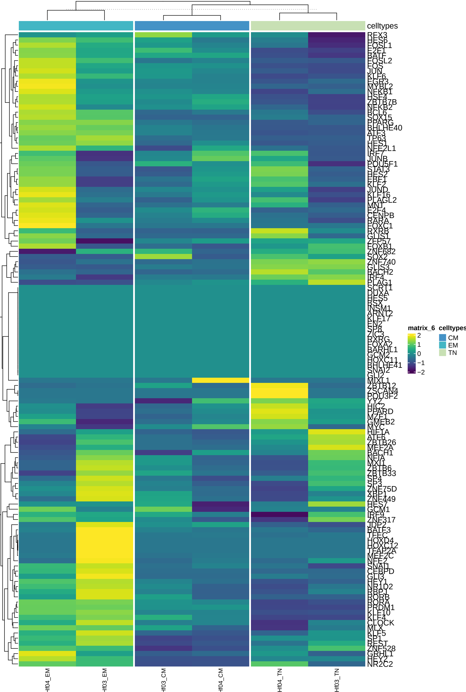
TF Gene Expression (FPKM, Row Z-Score)
