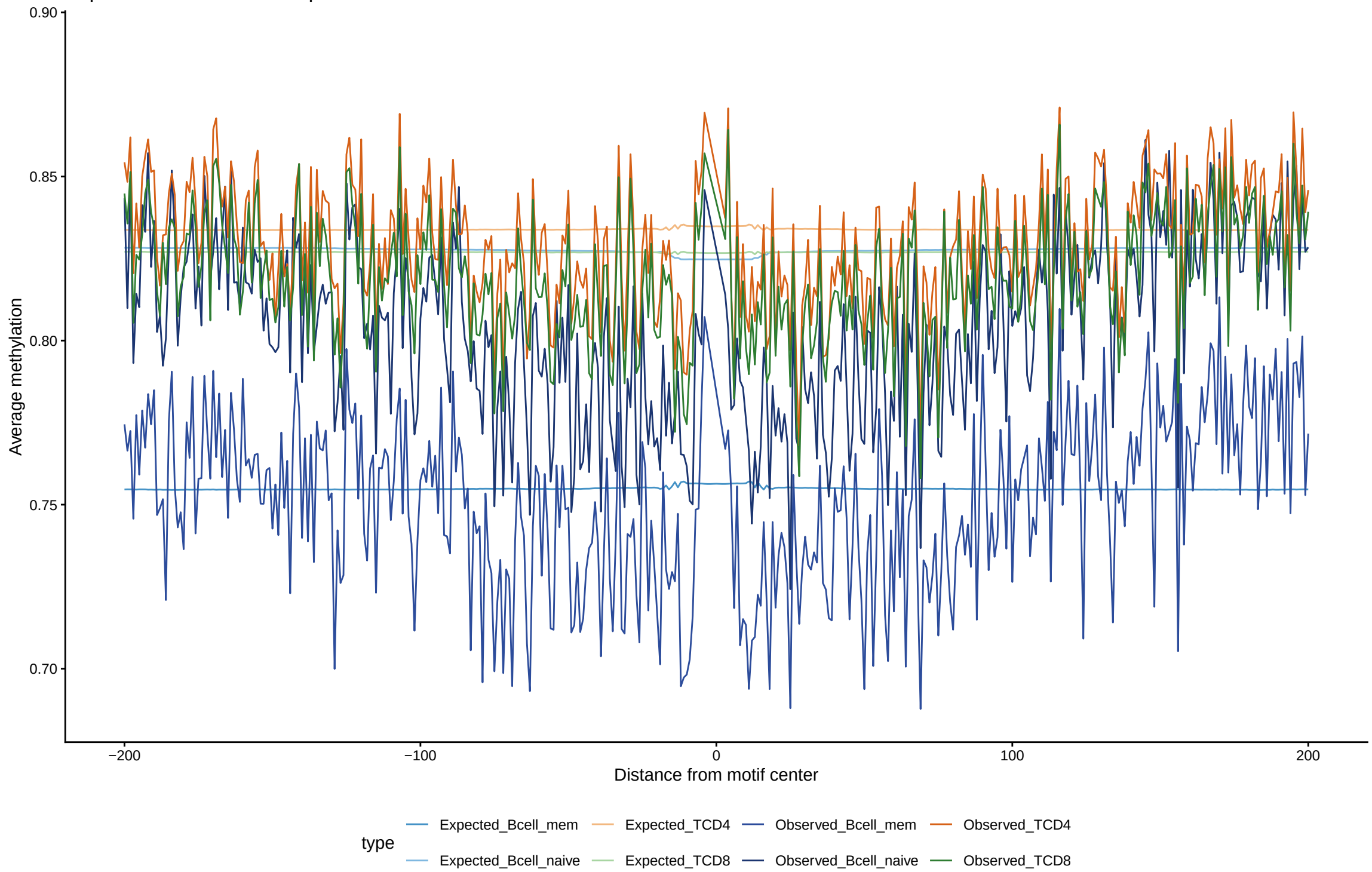
Expected vs observed footprints for MYOG
