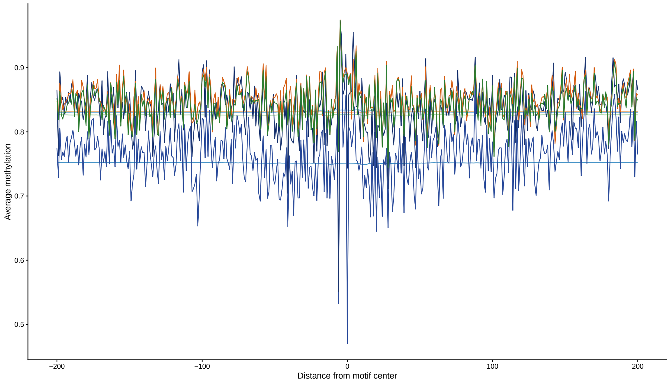
Expected vs observed footprints for PAX6
