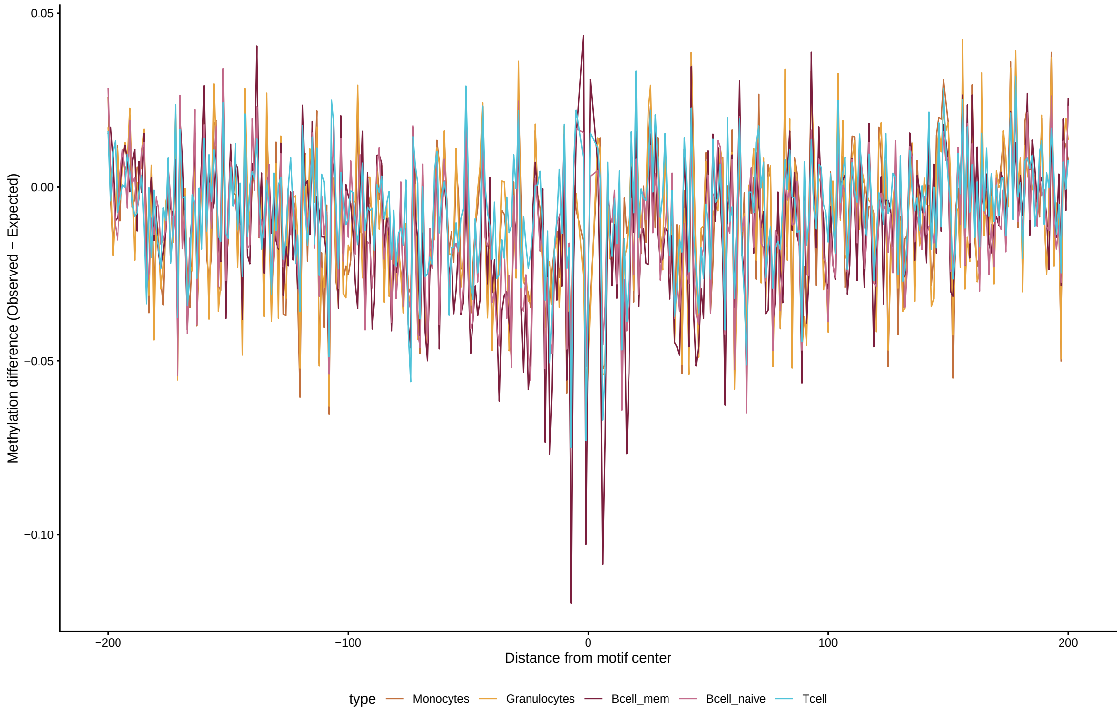
TF footprint difference for TFAP2E
