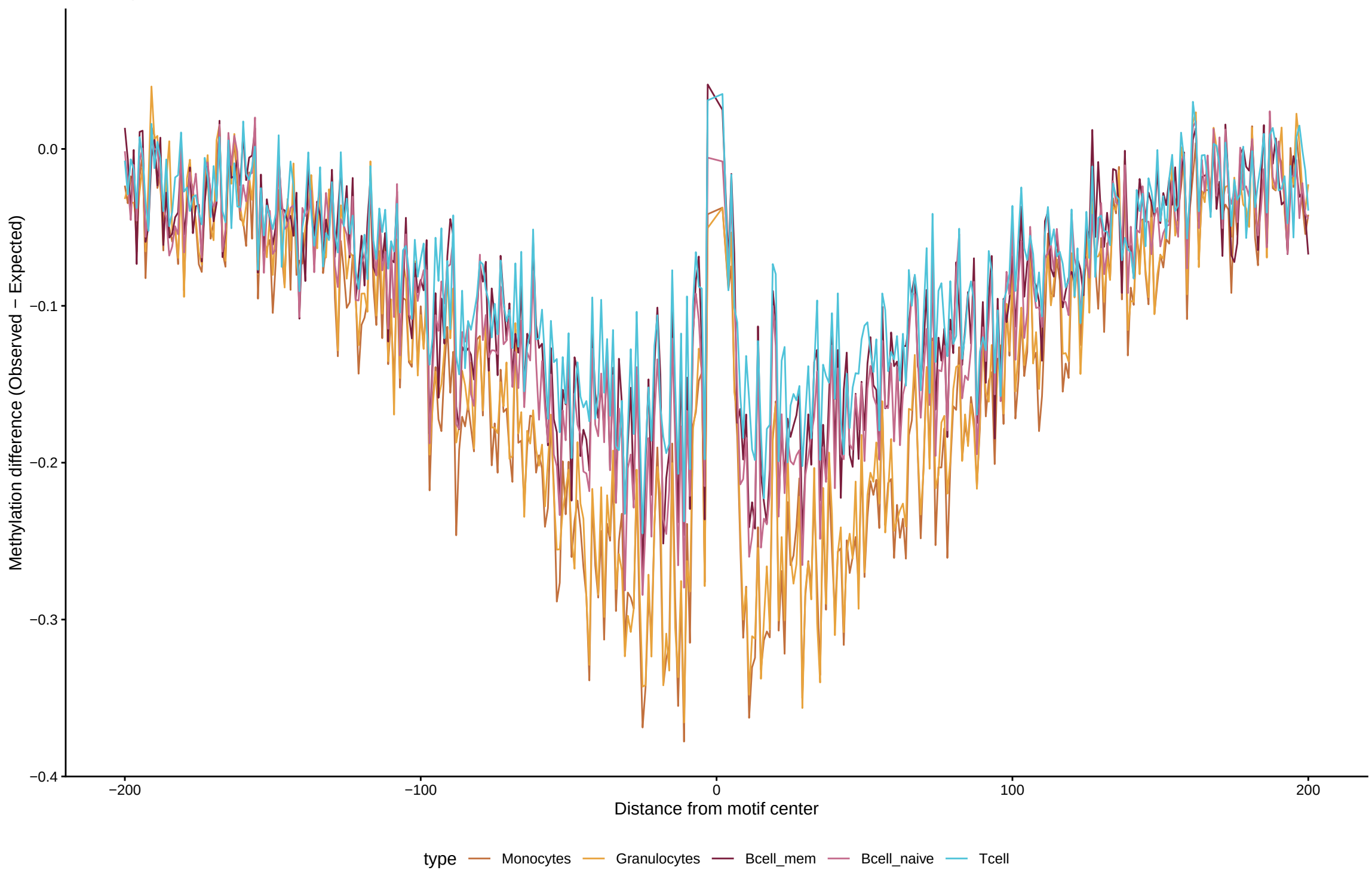
TF footprint difference for ETV5
