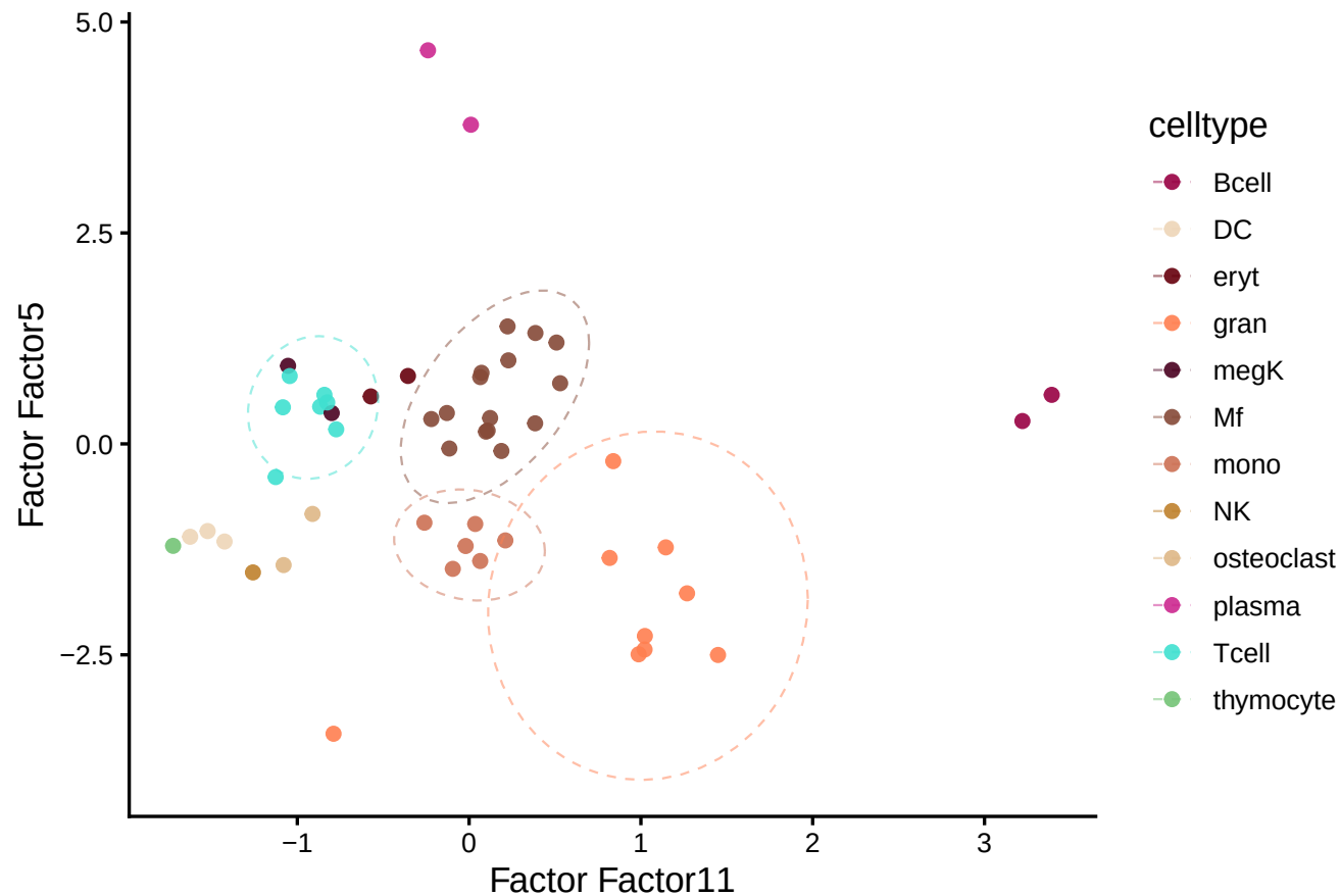
MOFA: Factor Factor11 vs Factor5 (colored by celltype)
