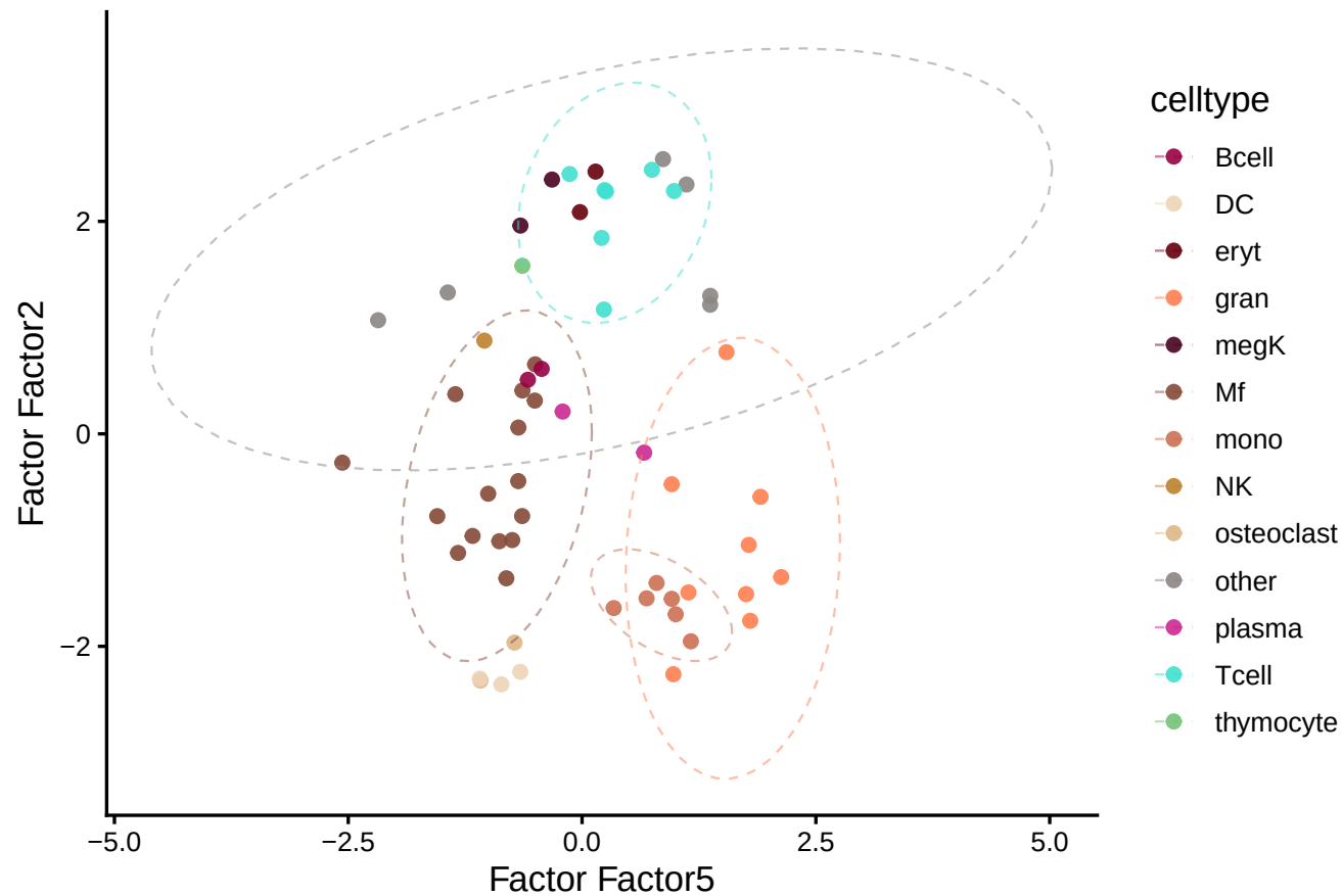
MOFA: Factor Factor5 vs Factor2 (colored by celltype)
