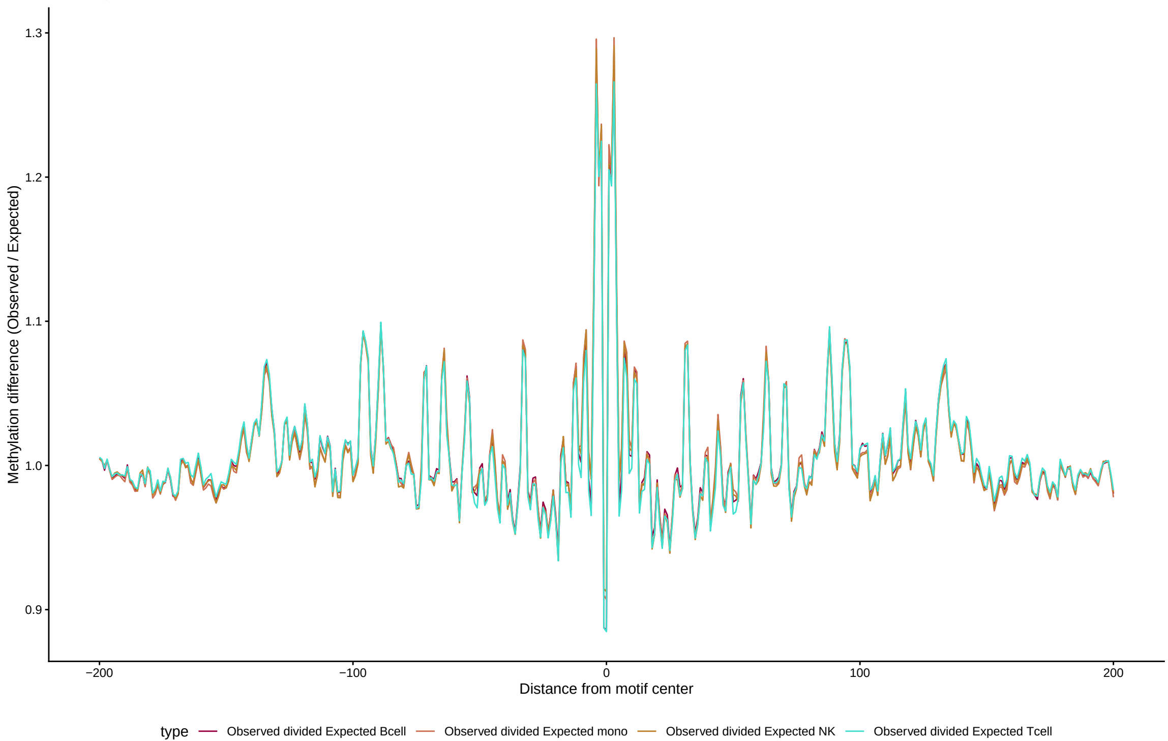
TF footprint difference for KLF4
