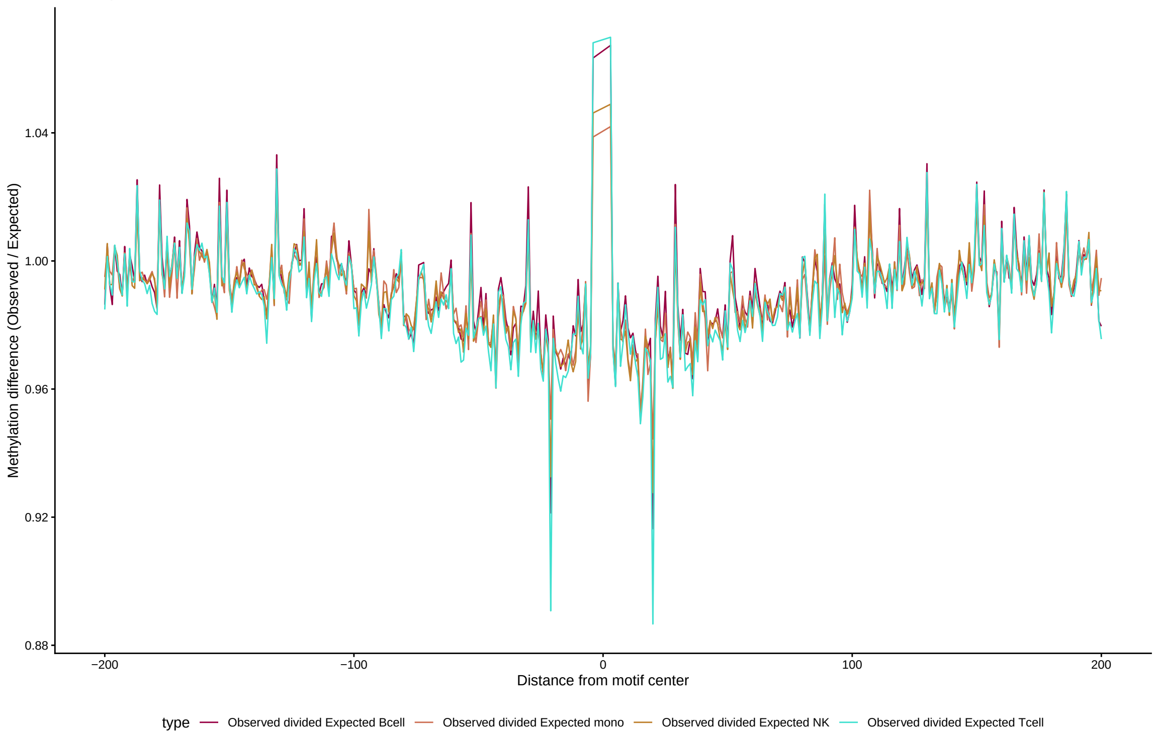
TF footprint difference for FOXP3
