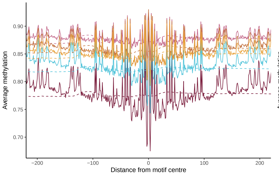
ap1_1 (1107575 sites)
