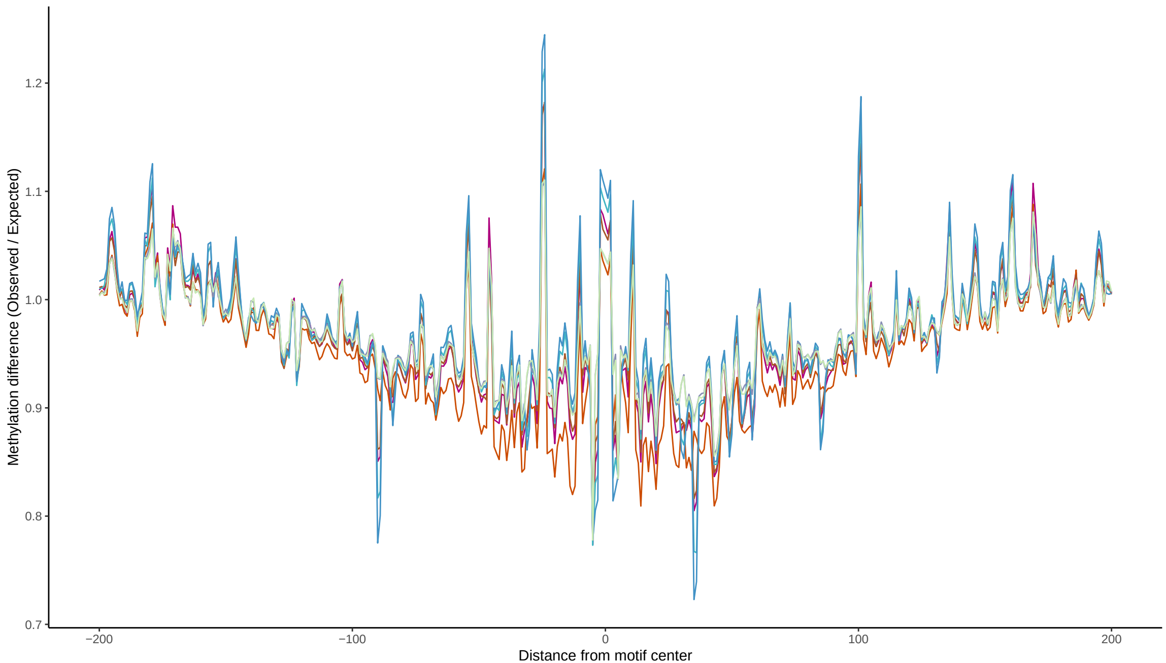
TF footprint difference for ELF5
