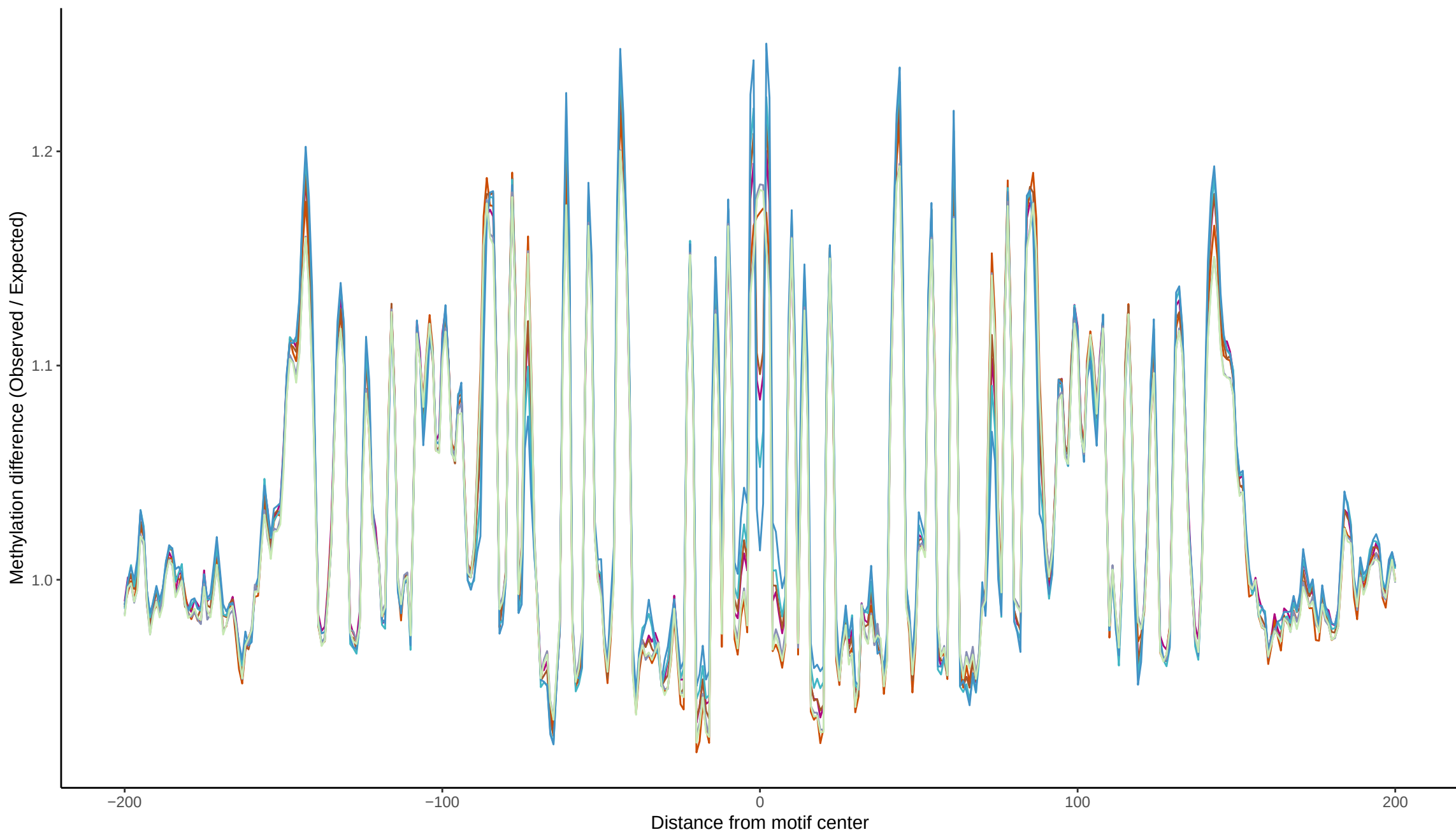
TF footprint difference for HES1
