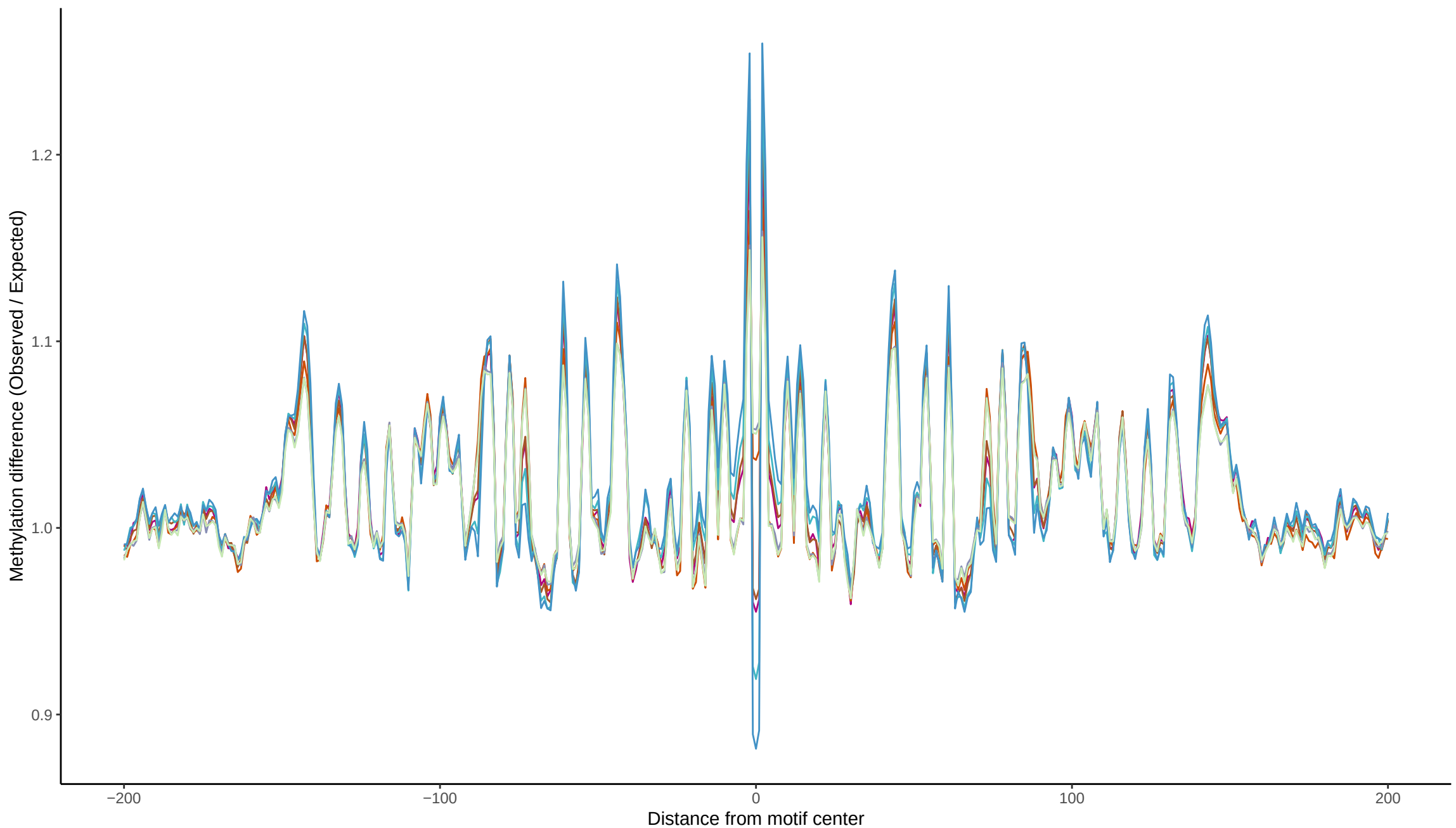
TF footprint difference for HEY1
