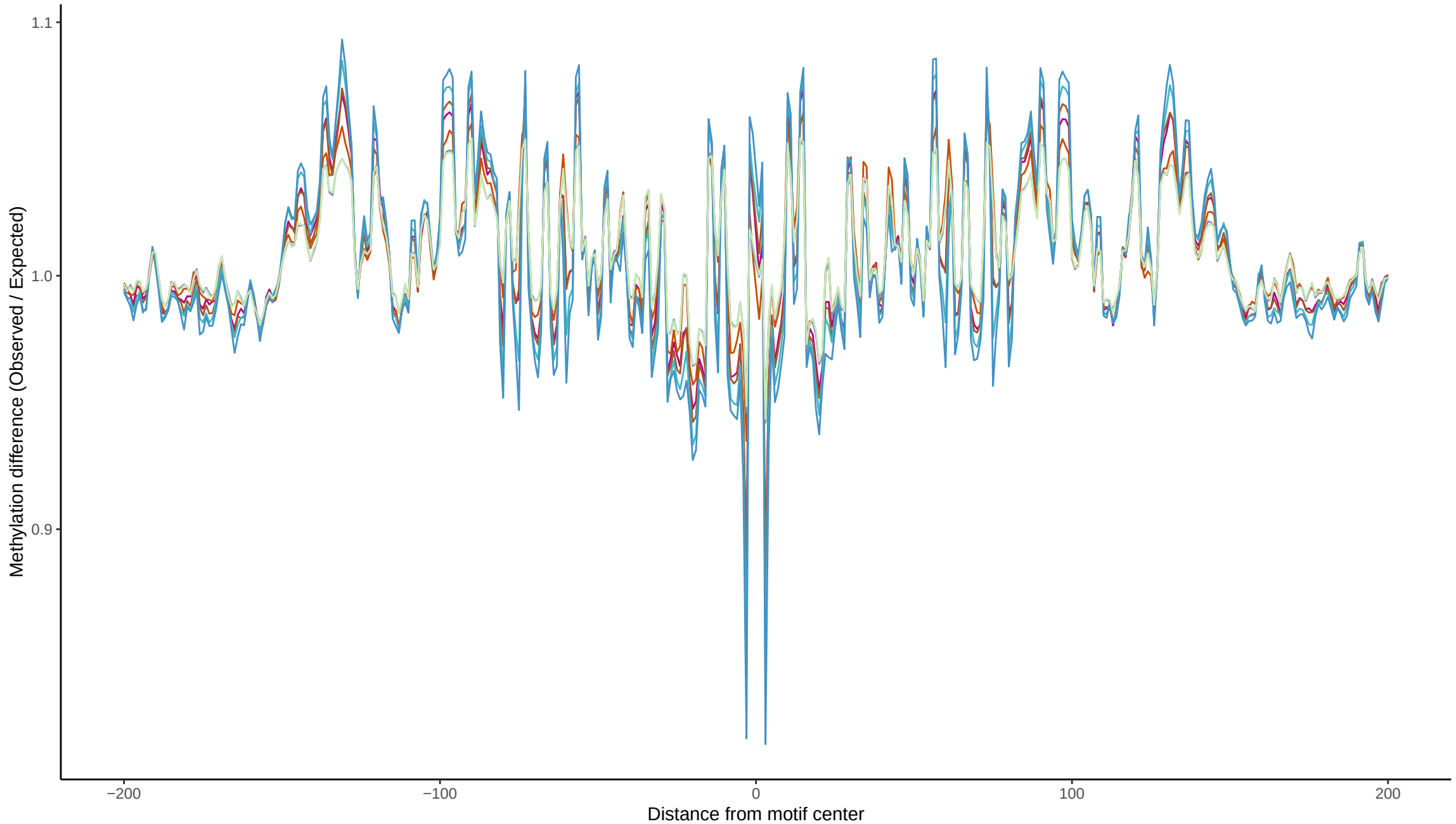
TF footprint difference for HIC2
