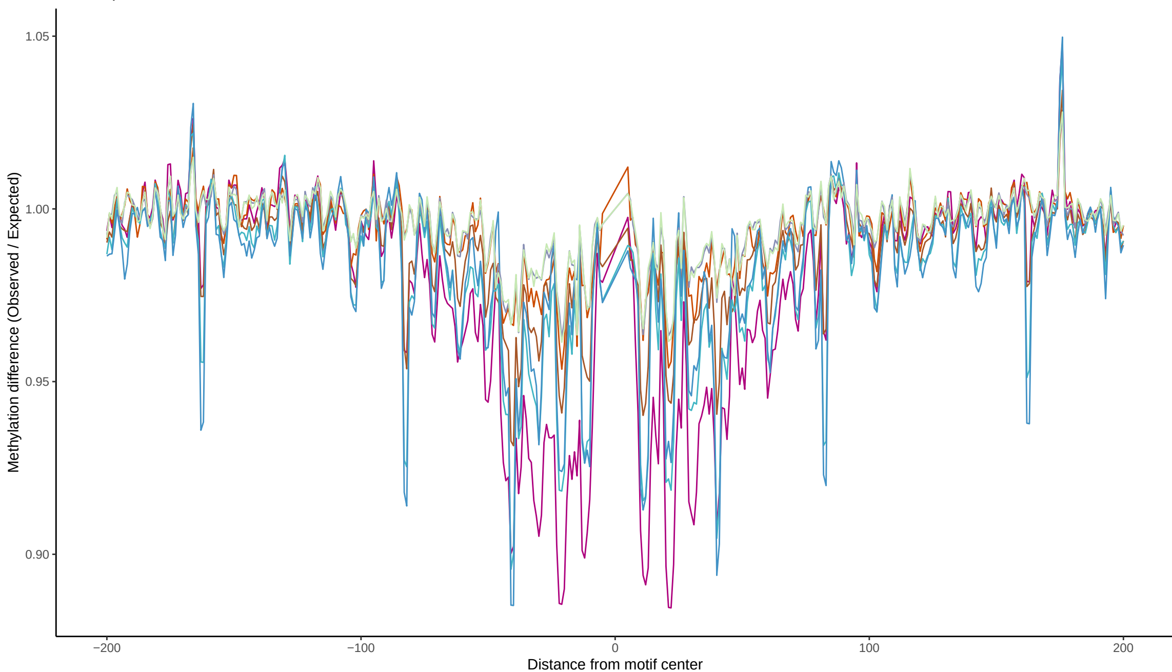
TF footprint difference for POU3F4
