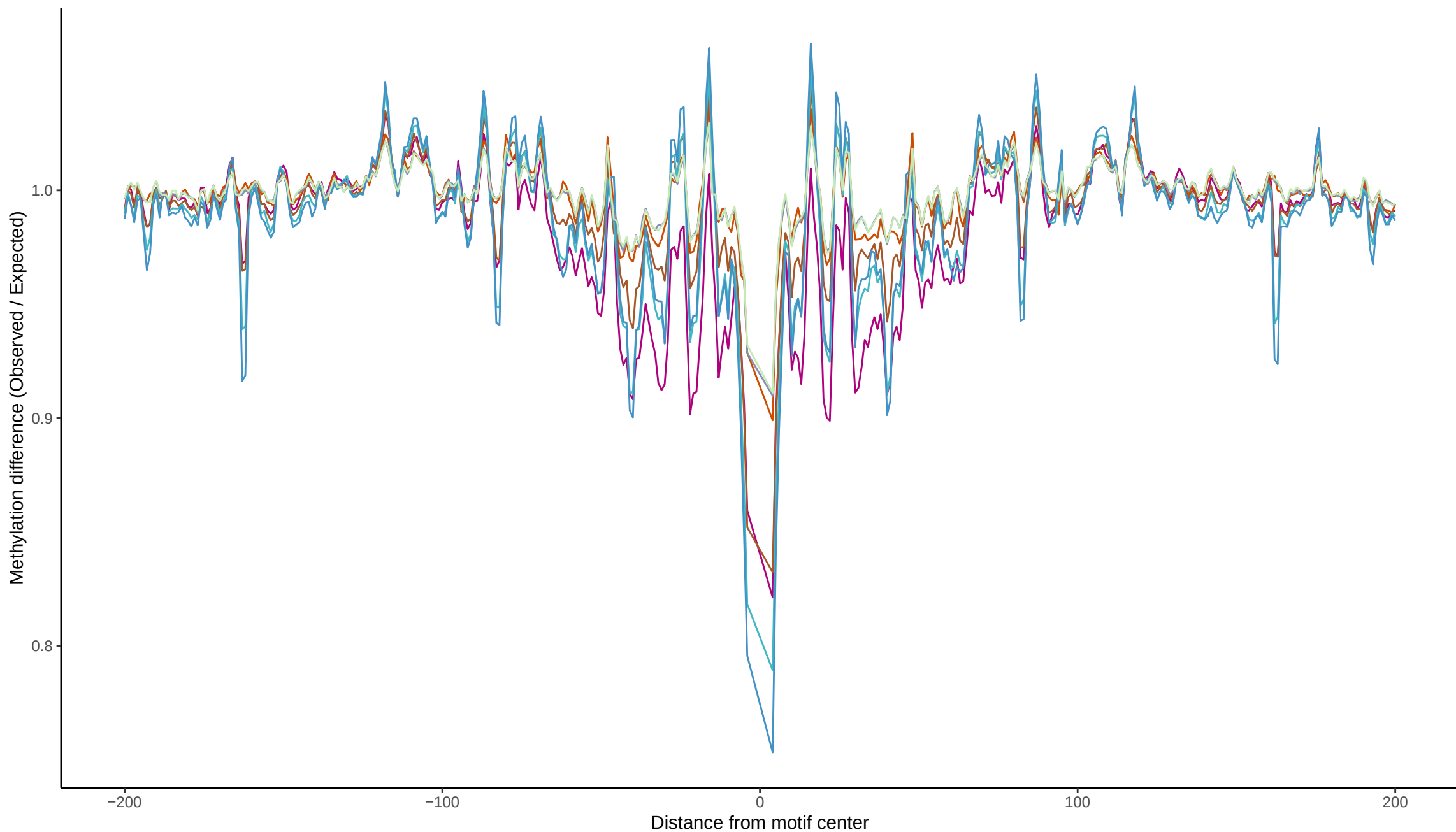
TF footprint difference for POU5F1
