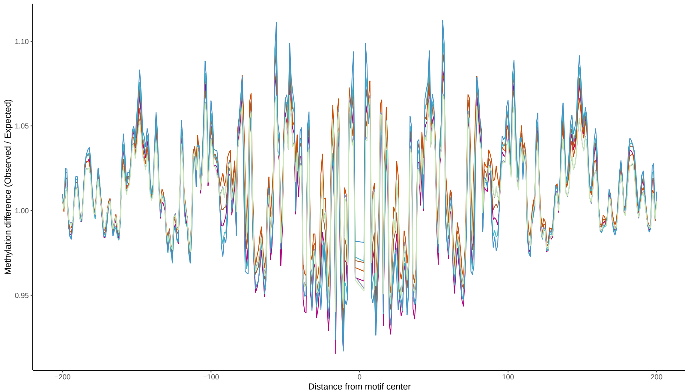
TF footprint difference for TCF4
