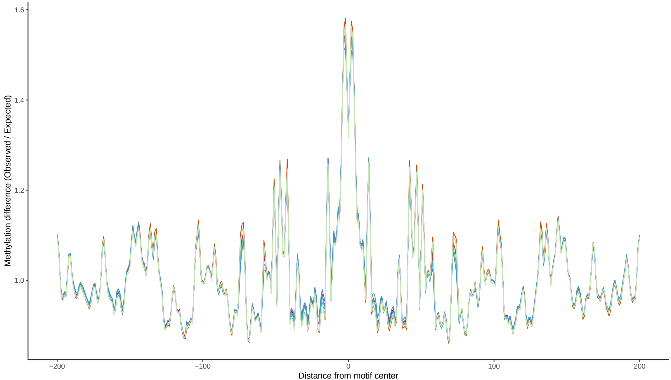
TF footprint difference for ZBTB14
