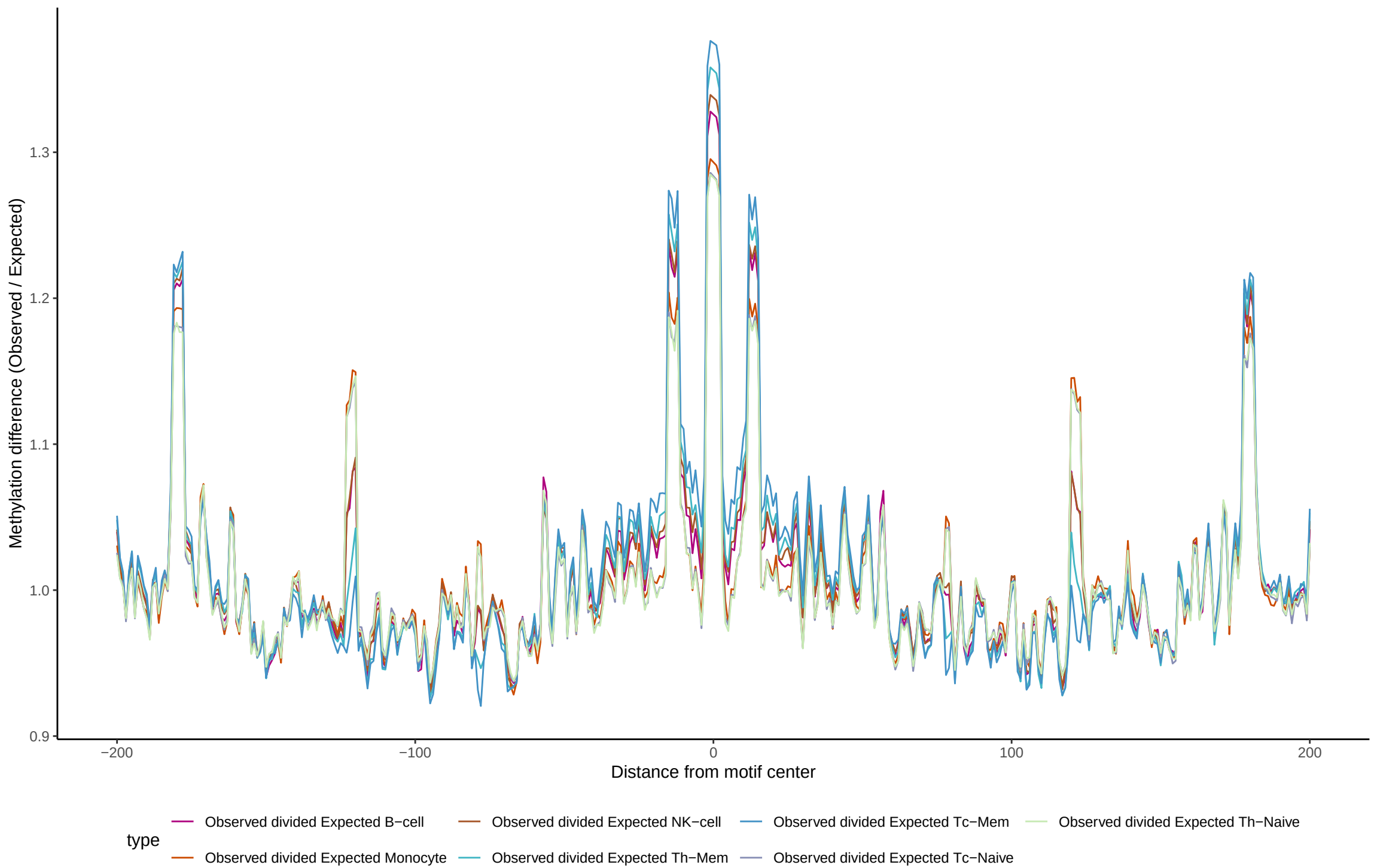
TF footprint difference for ZFP57
