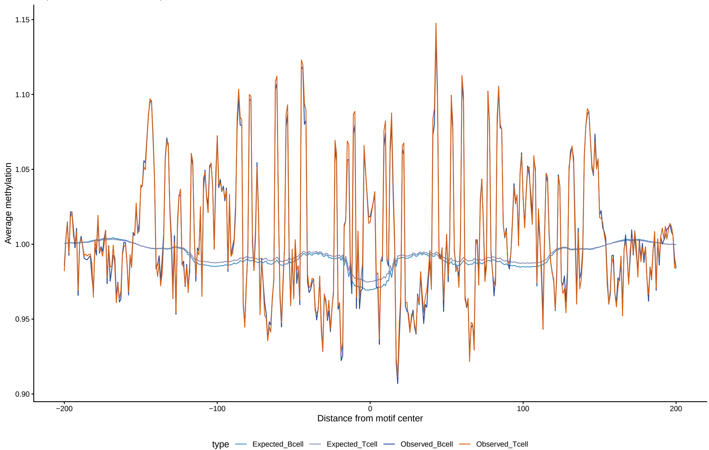
Expected vs observed footprints for ARNT2
